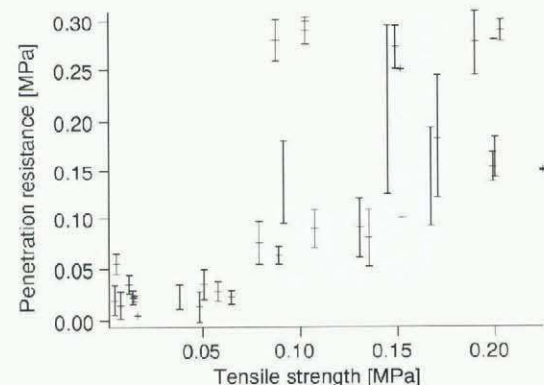
Fig. 6. Tensile strength and penetrometer resistance. The bars indicate the variation of the penetration tests surrounding the samples taken for tensile strength.
