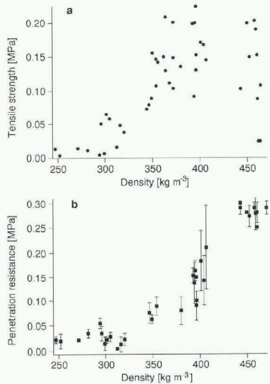
Fig. 5. Comparison between bulk density and tensile strength (a) and between bulk density and penetrometer resistance (b). The bars indicate the variation of the penetration tests surrounding the samples taken for tensile-strength testing. They also show the variability of the snow within about a 10 cm spacing.
