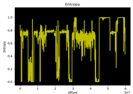
Figure 8. Entropy Analysis of Firmware
