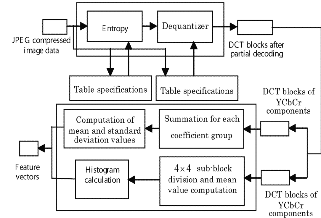
FIGURE 4. Feature vector extraction process
