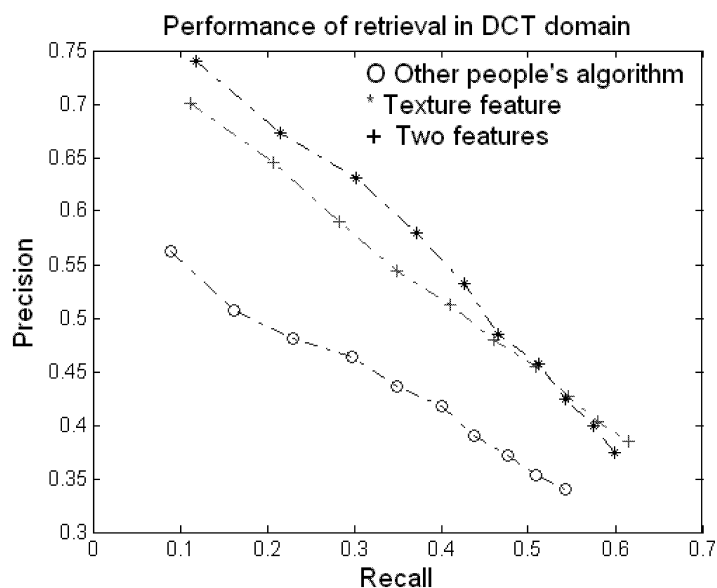
FIGURE 6. Comparisons of the retrieval performance
