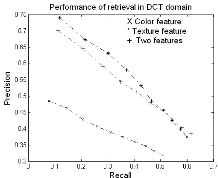
FIGURE 5. Retrieval performance comparisons for three cases
