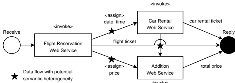
Figure 4: View of the original business process
