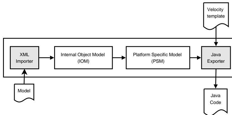
Figure 6: Model-driven Web service generator
