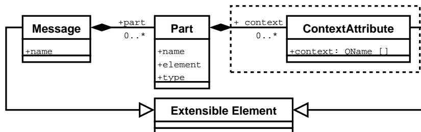
Figure 3: Partial representation of the extended WSDL meta-model
