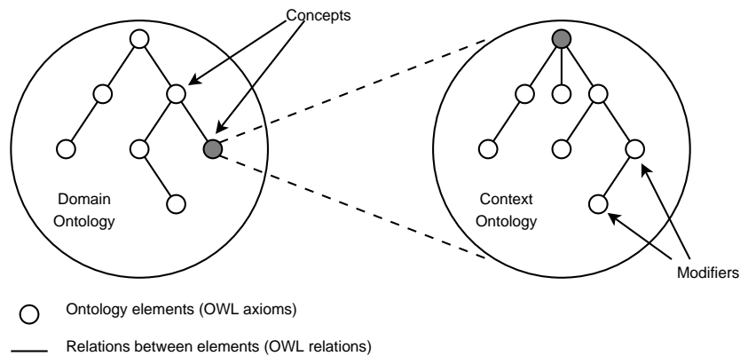
Figure 2: Context vs. domain ontologies
