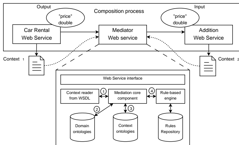
Figure 7: Detailed View of the Mediator Web service
