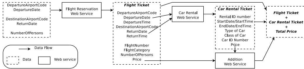
Figure 1: Flight-booking and car-rental Web services
