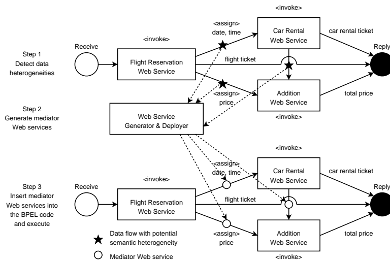
Figure 5: Generation of the mediator Web service
