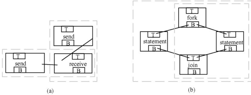
FIGURE 10. Examples of checking the selection-free condition.
