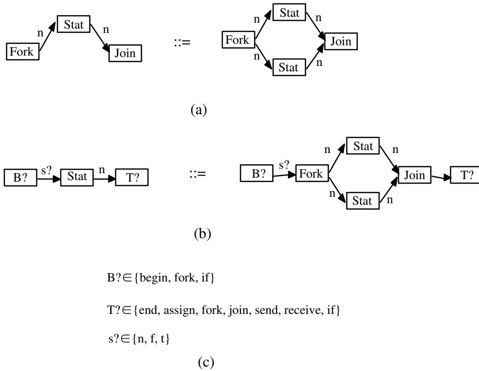
FIGURE 13. Productions in a LGG with different embedding mechanisms.
