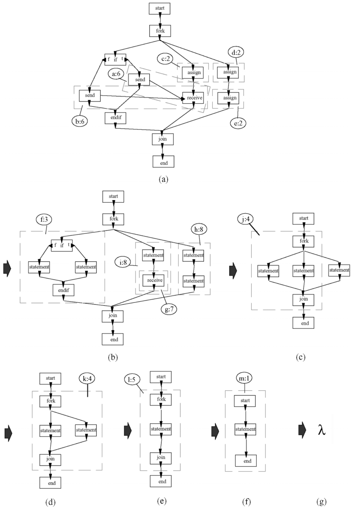
FIGURE 8. Graph transformations (parsing) when productions are applied.
