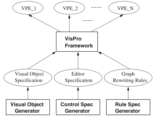
FIGURE 12. Constructing VPEs with VisPro.
