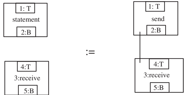
FIGURE 5. A graph rewriting rule.
