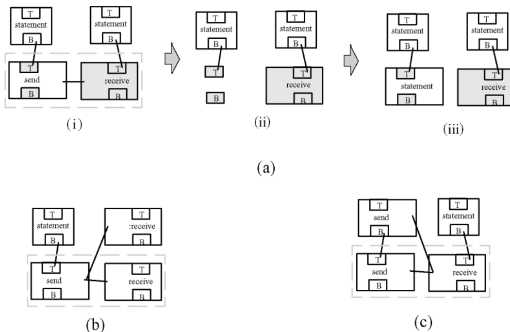
FIGURE 6. Examples of the R-application.
