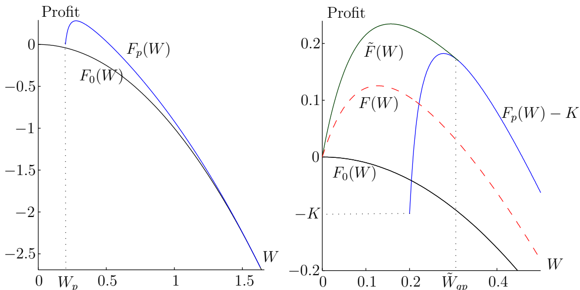
Figure 4: The principal's profit with promotion when \theta = 1.25 and K = 0.1 .
