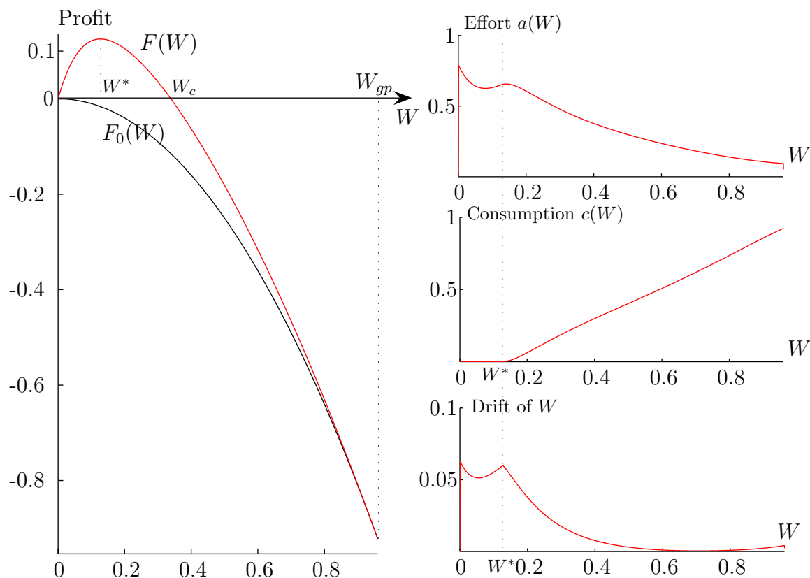
Figure 1: Function F for u(c) = \sqrt{c} , h(a) = 0.5a^2 + 0.4a , r = 0.1 and \sigma = 1 . Point W^* is the maximum of F .
