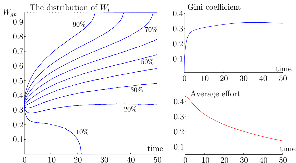
Figure 2: Consumption, inequality and expected output for the example in Figure 1.
