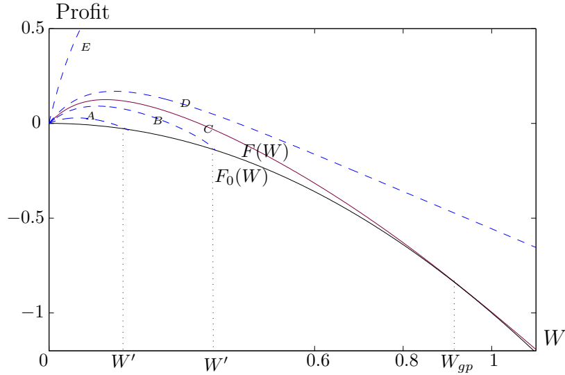
Figure 6: Typical solutions of the HJB equation.
