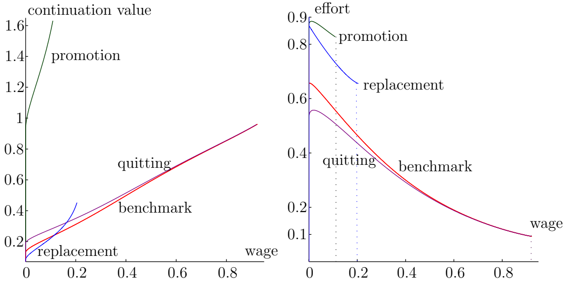
Figure 5: The agent's value and effort as functions of wage under different contractual possibilities.
