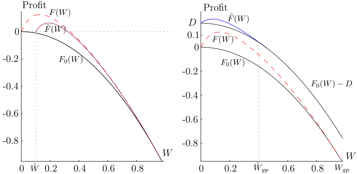
Figure 3: The principal's profit when the agent has an outside option of \tilde{W} = 0.1 (left panel) or the principal can replace him for profit D = 0.2 (right panel).
