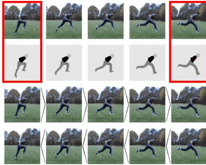
Figure 14: Top: Real frames from a video sequence. Middle: Discrete geodesic between the first and the last segmented frames. Bottom rows: Pullback of the last frame (top) and pushforward (bottom) of the first one (the background has been pasted into the pullbacks and pushforwards so that it is not deformed).
