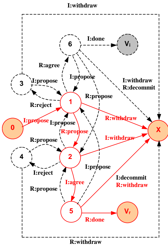
Figure 3. The Contract Net protocol derived from the general interaction protocol
