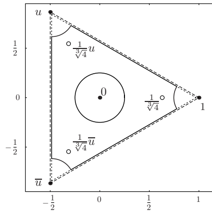
FIGURE 6. z - z^4
