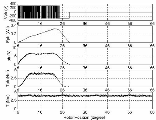
(c) Actual profiles at the speed = 800 rpm
