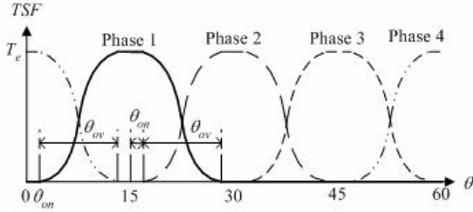
Fig. 1 Typical profile of the proposed TSF for a four-phase SRM drive
