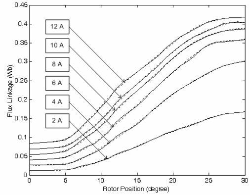
Fig. 3 Given and computed flux linkage characteristics for the four-phase SRM drive
