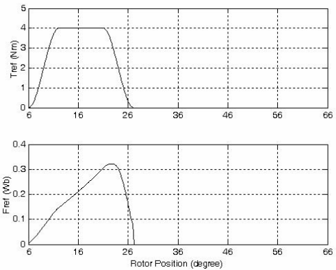
(a) Torque and flux linkage references
