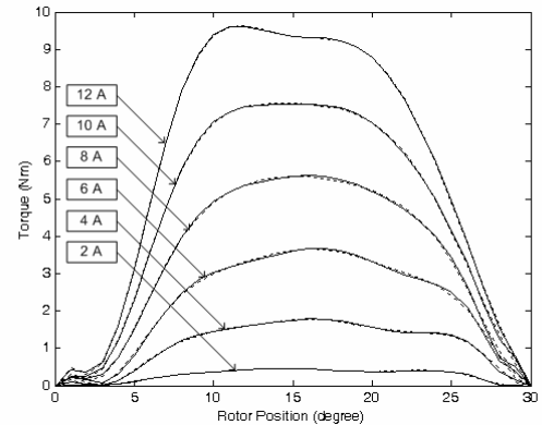
Fig. 4 Given and computed static torque characteristics for the four-phase SRM drive
