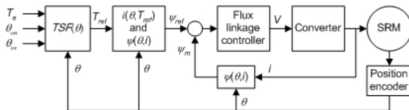
Fig. 2 Structure of the proposed control scheme of torque ripple minimization based on the flux controller
