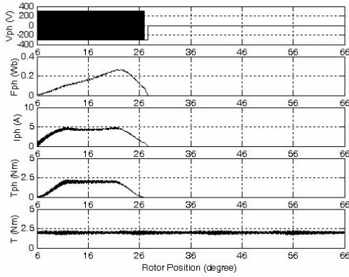
(b) Actual waveforms at the speed = 400 rpm
