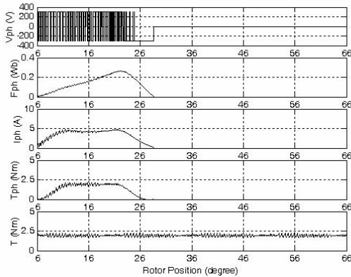
(c) Actual waveforms at the speed = 1000 rpm
