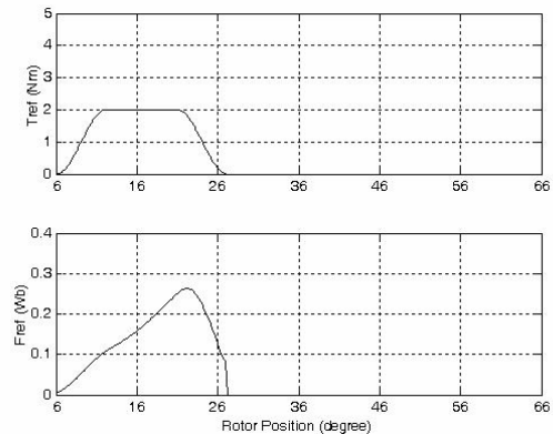
(a) Torque and flux linkage references
