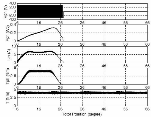
(b) Actual profiles at the speed = 200 rpm
