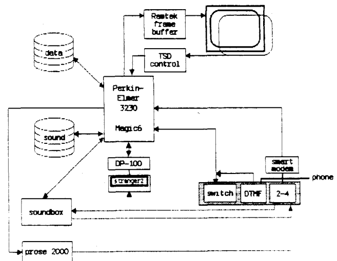
Figure 2: Hardware configuration used in Phone Slave.
