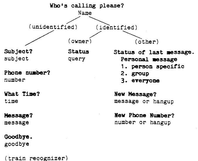
Figure 1: Tree of possible conversations.
