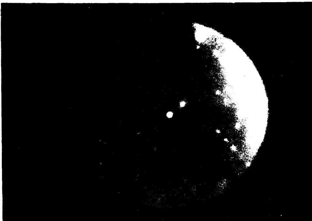
C_2N_2 on Ni(111)
