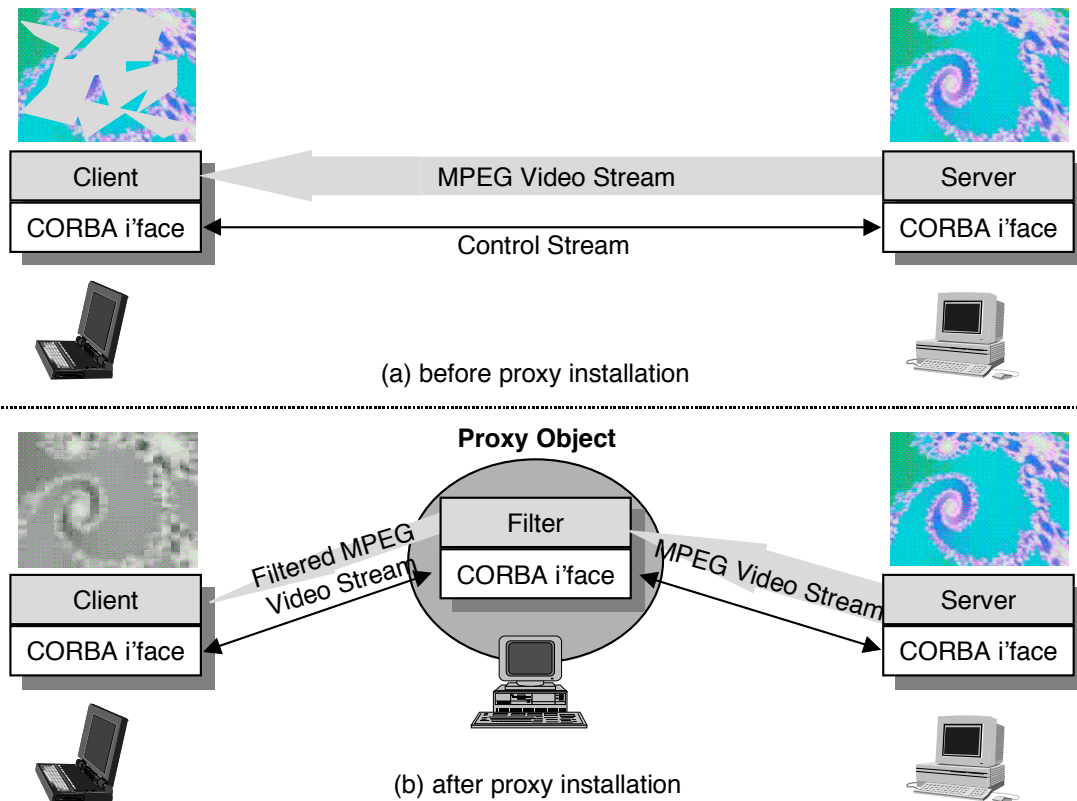
Figure 7. Installing a Proxy Object
