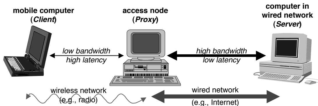
Figure 1. Example of a Proxy
