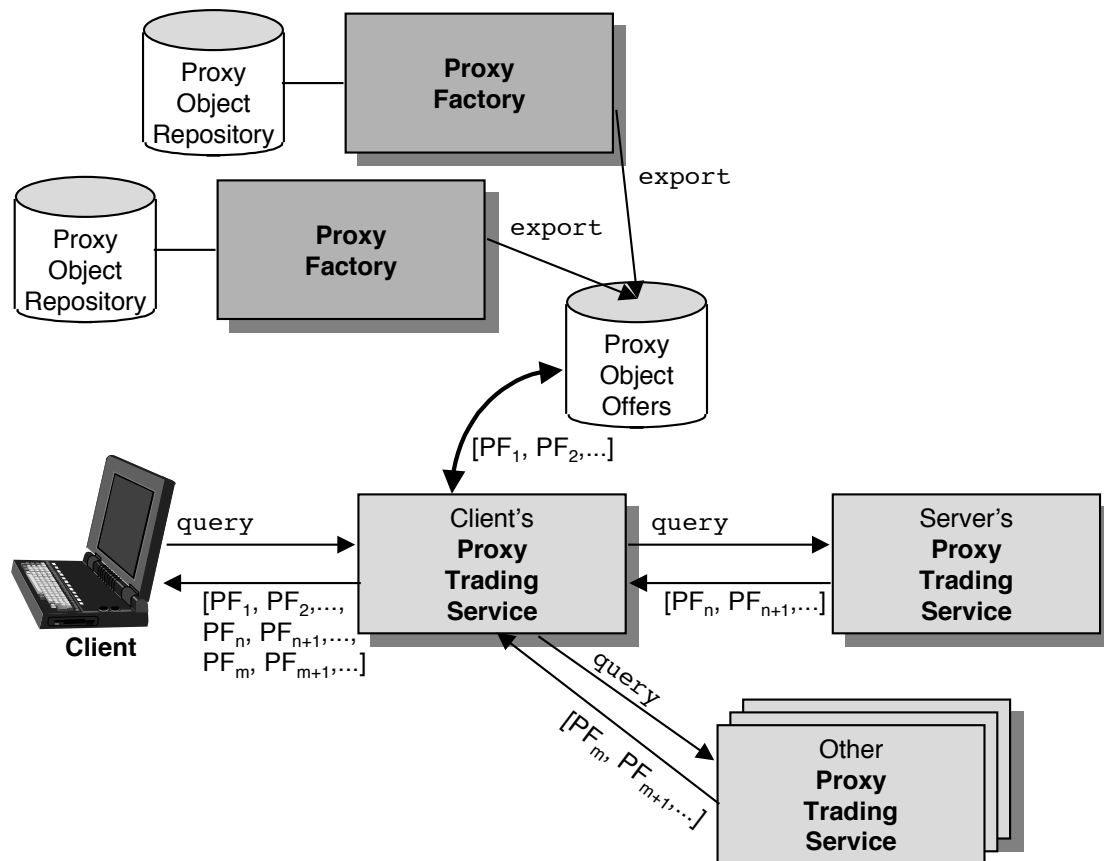
Figure 4. The Proxy Trading Service
