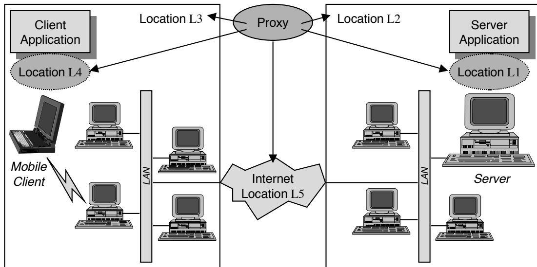
Figure 3. Options of Proxy Placement
