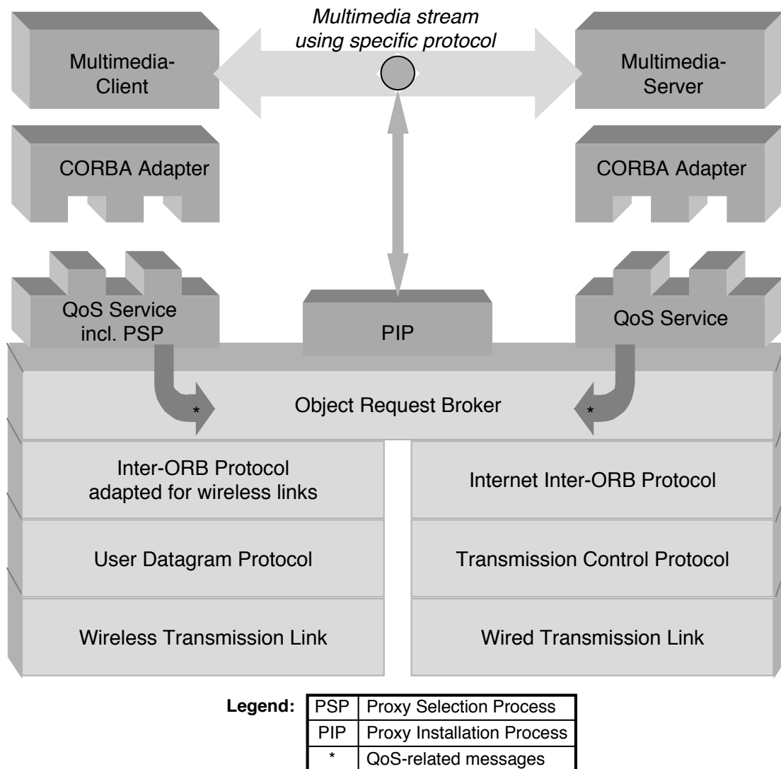
Figure 2. The RAPP Architecture
