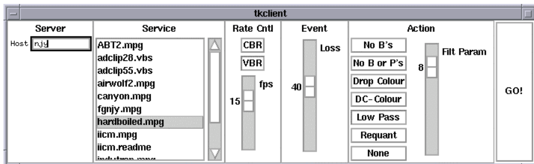
Figure 5. Client Application Control Panel
