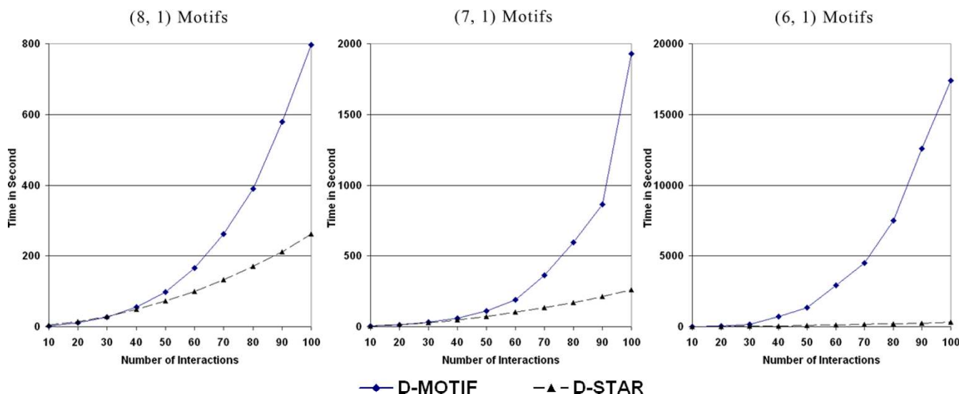
Figure 8 Comparison of running time between D-MOTIF and D-STAR. Observe that the running time of D-MOTIF increases rapidly as the input data grows and also as the (l, d) -motif gets weaker. All experiments were run on a x86 Pentium 4 1.6 GHz machine with 512 MB of memory.
