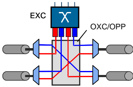
Figure 7: Hybrid transparent node architecture integrating an all-optical cross-connect and an EXC
