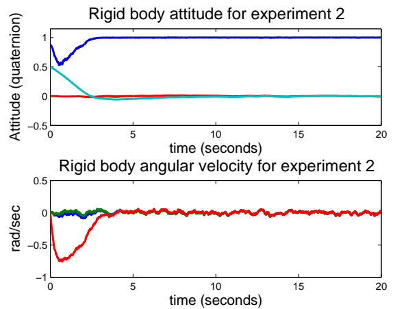
Figure 4: The simulated attitude and angular velocity using only the acceleration directional measurements
