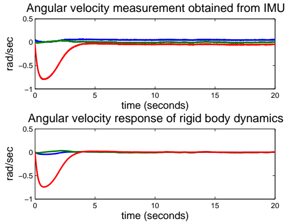
Figure 2: The evolution of the IMU measured values (top) and the true values of angular velocity for the rigid body dynamics. Note that the measured values in the top graph show a constant bias. This is compensated for the combined control design.
