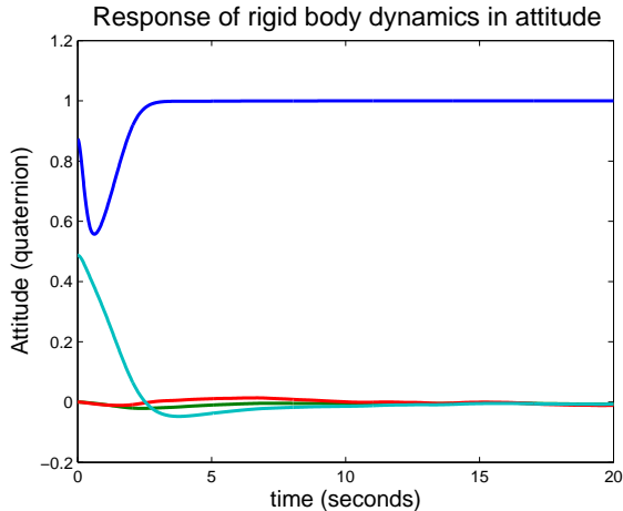
Figure 1: The evolution of the quaternion state for experiment one. The desired set point is (1, 0, 0, 0) . Due to the noise model, only practical convergence to a neighbourhood of the desired set point is observed.
