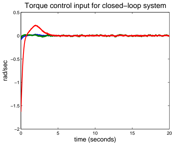
Figure 3: The simulated control input to the rigid body dynamics
