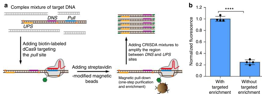
Fig. 6 Targeted enrichment of DNA by Cas9 further enhances the sensitivity of CRISDA. a Schematic of the Cas9-mediated specific enrichment of target DNA in combination with CRISDA. b Representative endpoint fluorescence measurements showing that the sensitivity and reliability of CRISDA are significantly enhanced when combined with Cas9-mediated enrichment of target DNA (reactions are conducted at an hTF1 concentration of 2.5 aM). In each replicate, fluorescence intensity of the CRISDA reaction without targeted enrichment were normalized against the one with targeted enrichment. n = 4 technical replicates, two-tailed Student's t test; **** P < 0.0001 , bars represent mean \pm s.d
