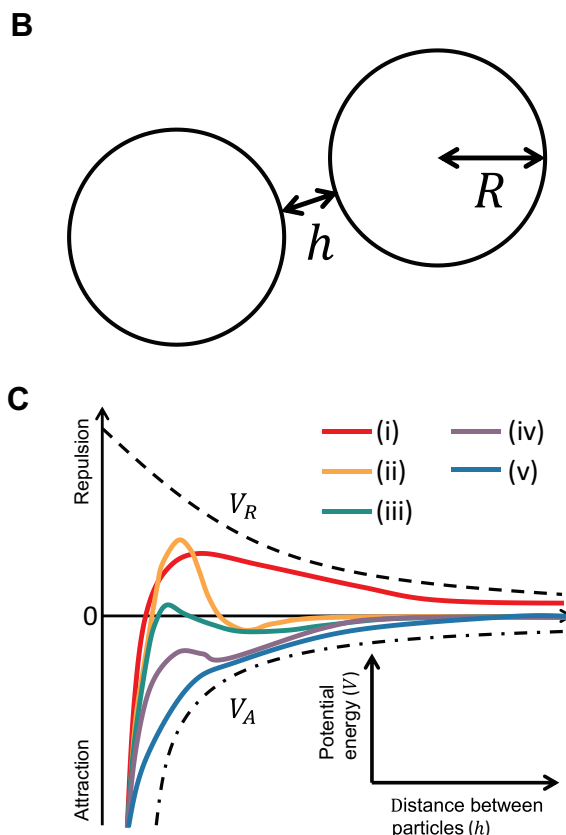
Figure 3 (A) Equations of the DLVO theory. (B) Relationship between two particles assuming the DLVO theory. (C) A typical example of potential energy presented in the DLVO theory.
