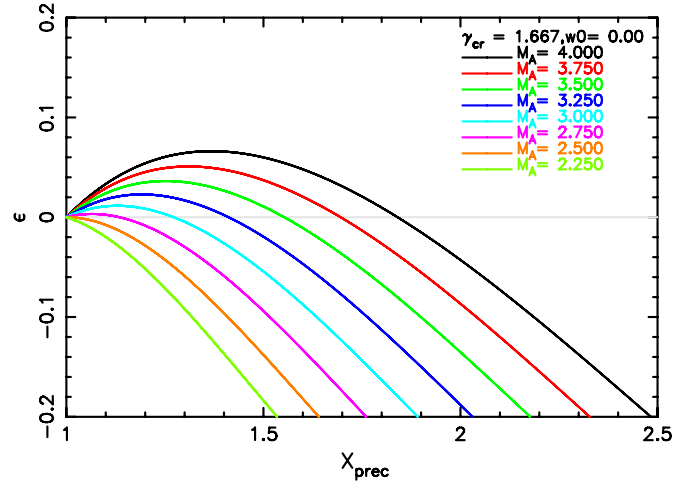
Figure 6. Same as Figure 1 (left), but now for perpendicular shocks with \beta_0 = 0 , and with Mach numbers that include the appropriate critical Alfvén Mach number M_A = 2.5 (orange).
