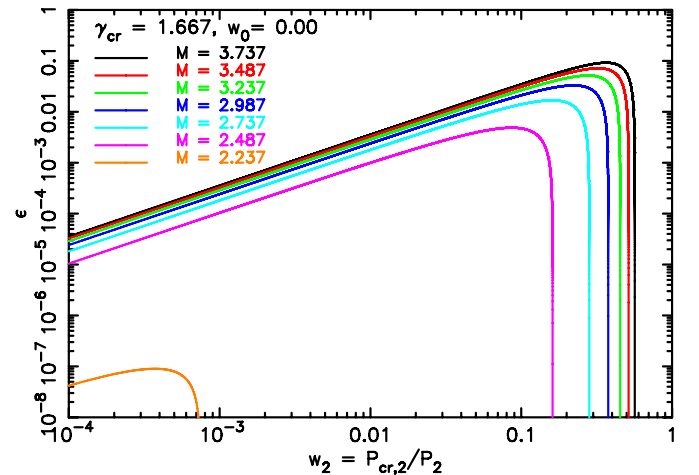
Figure 2. Solutions to two-fluid model of Vink et al. (2010). The values for the Mach number correspond to those in Figure 1, except that the orange curves correspond to M_{g,0} = \sqrt{5} + 0.001 , in order to show the behavior very close the critical Mach number.
