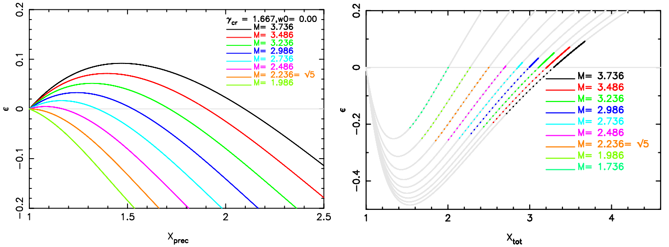
Figure 1. Left panel: the curves represent the solutions of the energy-flux escape parameter \epsilon as a function of the precursor compression ratio \chi_{\text{prec}} , for various values of the overall Mach number, with increments of \Delta M_{g,0} = 0.25 . The slopes at \chi_{\text{prec}} = 1 are negative for M_{g,0} < \sqrt{5} , resulting in negative values of \epsilon , which is unphysical. For M_{g,0} > \sqrt{5} one does obtain physical solutions, but energy escape is required ( \epsilon > 0 ). Right panel: the behavior of \epsilon as a function of total shock compression \chi_{\text{tot}} (Equation (A15)) for the same Mach numbers as in the left panel. The total, light gray, curve shows a wide range of shock compression ratios, but only values \epsilon \geq 0 correspond to potentially physical solutions. The colored curves are solutions to the two-fluid model of Vink et al. (2010), with the unphysical solutions ( \chi_{\text{prec}} < 1 ) indicated with a dotted line. The highest values of \chi_{\text{tot}} of the colored lines correspond to the maximum compression ratios as given by Equation (1). The compression ratios with \epsilon = 0 correspond to the standard Rankine–Hugoniot solutions. (A color version of this figure is available in the online journal.)
