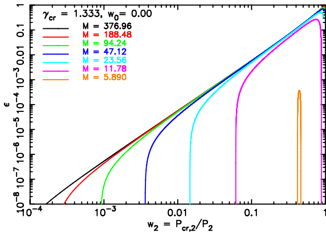
Figure 3. Same as Figure 2, but now for an accelerated particle component characterized by \gamma_{\text{cr}} = 4/3 , for logarithmically spaced intervals of the Mach number.
