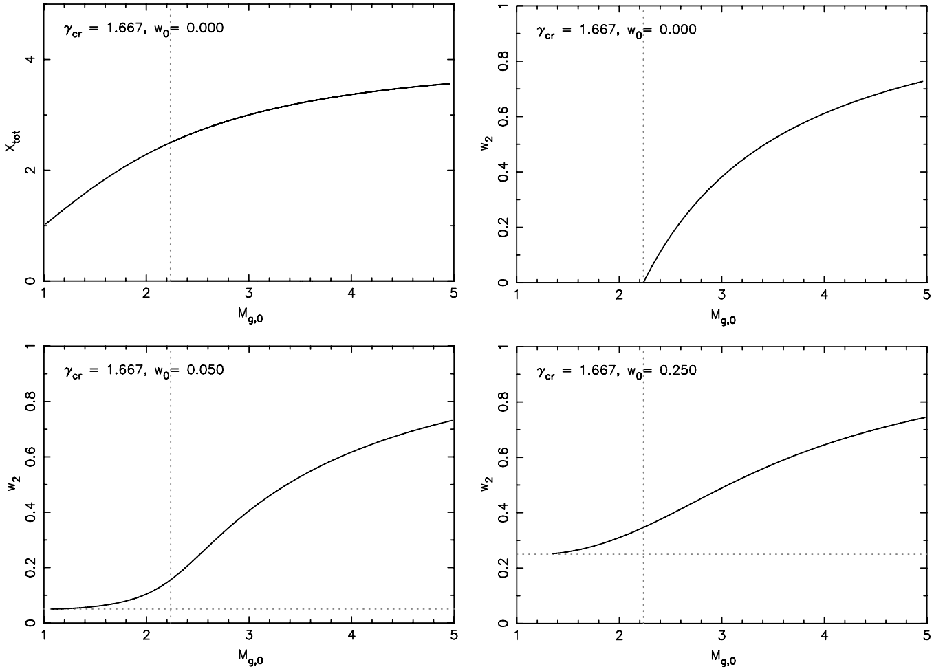
Figure 9. Shock solutions for \gamma_{\text{cr}} = 5/3 as a function of Mach number M_{g,0} for the case in which no energy is escaping from the system ( \epsilon = 0 ), corresponding to the two-fluid model of Drury & Voelk (1981). Top left panel: the total compression ratio, which follows the standard Rankine–Hugoniot relations for \gamma = 5/3 . Other panels: the downstream fractional cosmic-ray pressure for increasing values of the pre-existing cosmic-ray fractional pressure: w_0 = 0, 0.05, 0.25 . The vertical dotted line indicates the critical acceleration Mach number M_{\text{acc}} = \sqrt{5} , whereas the horizontal dotted line indicates w_0 . Note that the total compression ratios can be higher for \epsilon > 0 , whereas the maximum values for w_2 provide upper bounds for \epsilon > 0 .
