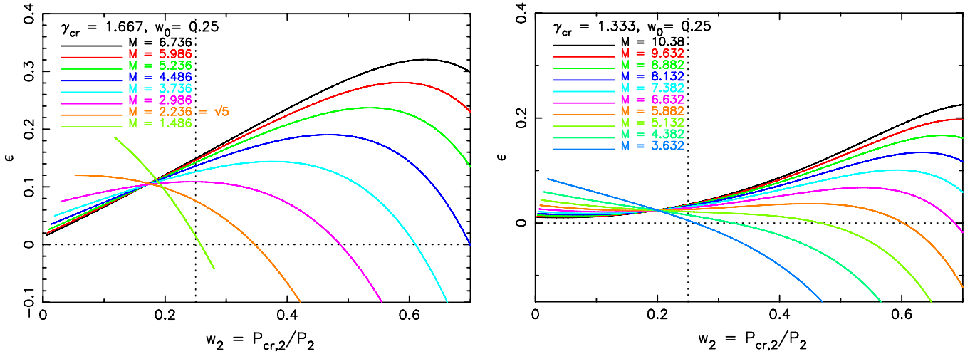
Figure 8. Solutions for the escape flux as a function of the downstream cosmic-ray pressure w_2 (similar to Figures 2 and 7), but now with the contribution of an additional upstream cosmic-ray pressure from pre-existing cosmic rays, w_0 = 0.25 (Equation (A15)). The left panel is for a non-relativistic accelerated particle population ( \gamma_{\text{cr}} = 5/3 ), the right panel is for relativistically dominated particles ( \gamma_{\text{cr}} = 4/3 ). The Mach numbers differ 0.75 (1.33) times an integer number from the critical Mach number, M_{\text{acc}} = \sqrt{5} for \gamma_{\text{cr}} = 5.3 and M_{\text{acc}} = 5.882 for \gamma_{\text{cr}} = 4/3 .
