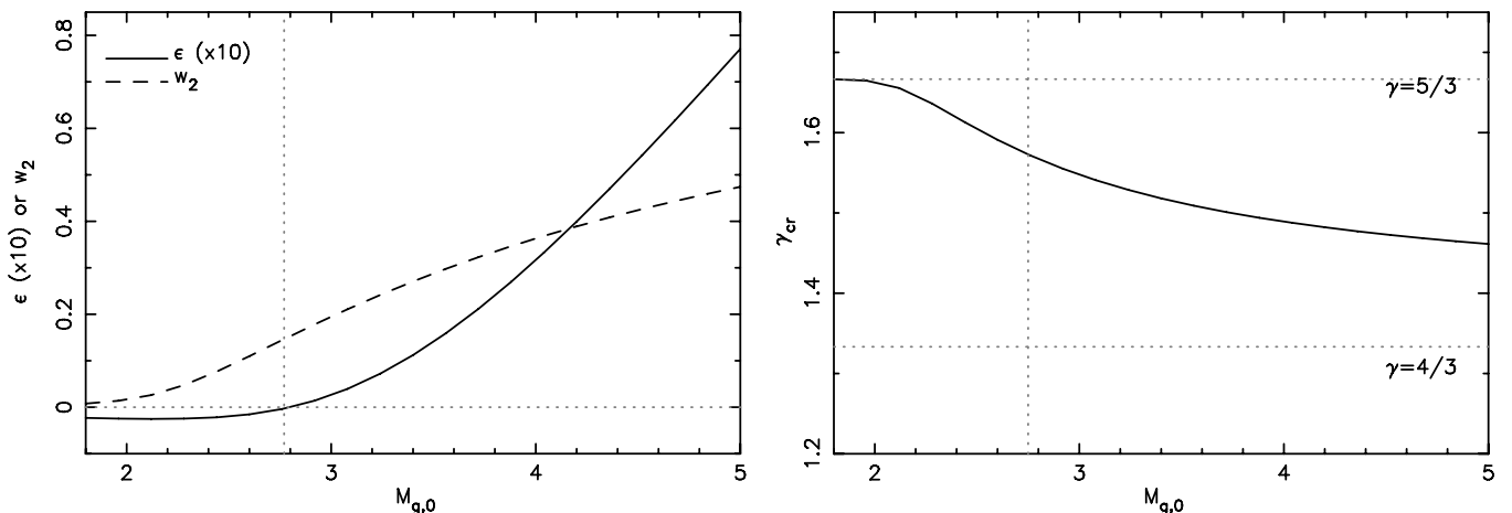
Figure 4. Shock solutions as obtained with the kinetic shock acceleration model of Blasi et al. (2005) for a shock velocity of V_s = 10 \text{ km s}^{-1} , and a maximum momentum of the accelerated particles of p_{\text{max}} = 100mc . Left: the values for the escape flux, \epsilon (multiplied by 10), and w_2 . Right: effective adiabatic index \gamma_{\text{cr}} of the accelerated particles. The limiting Mach number for this case is M_{\text{acc}} \approx 2.79 .
