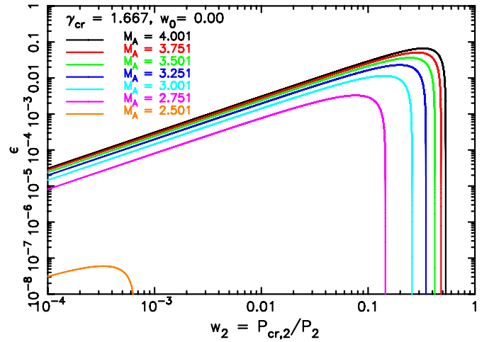
Figure 7. Same as Figure 2, but now for perpendicular shocks with \beta_0 = 0 , and with Mach numbers that include a value close to the critical Alfvén Mach number M_A = 2.5 (orange).
