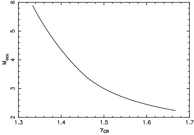
Figure 5. Critical Mach number as a function of assumed adiabatic index for the accelerated particle population ( 4/3 \leq \gamma_{\text{cr}} \leq 5/3 ).
