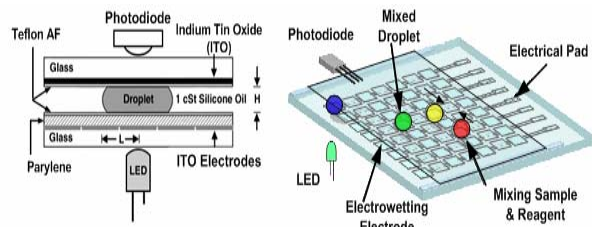
Fig. 1: Schematic diagram of a digital microfluidic biochip.
