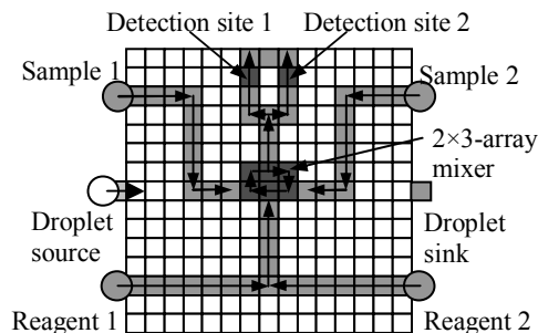
Fig. 10: A 15 \times 15 array used for multiplexed bioassays.
