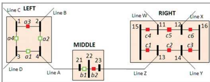
Figure 3. Line status determination from breaker status
