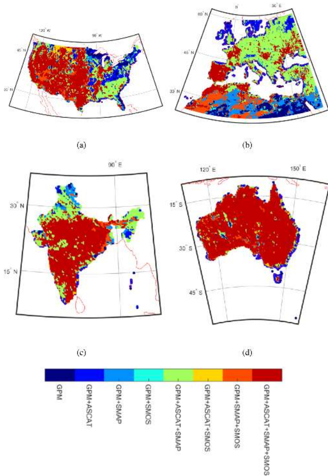
Figure 3. Products used in the integration over CONUS (a), Europe (b), India (c) and Australia (d). The results refer to 2015–2017 period.
