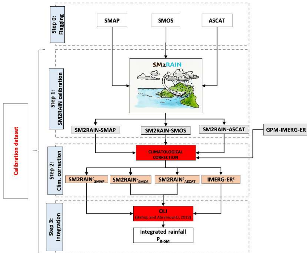
Figure 1. Integration scheme used for the calculation of the integrated rainfall product P_{R+SM} . In step 2, SM2RAIN c SMAP , SM2RAIN c SMOS , SM2RAIN c ASCAT and IMERG-ER c refer to the SM2RAIN products with climatological correction (using the calibration dataset).
