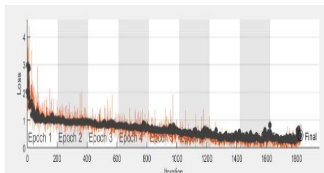
FIGURE 12. Loss in accuracy process of 3D- view w/o augmentation.
