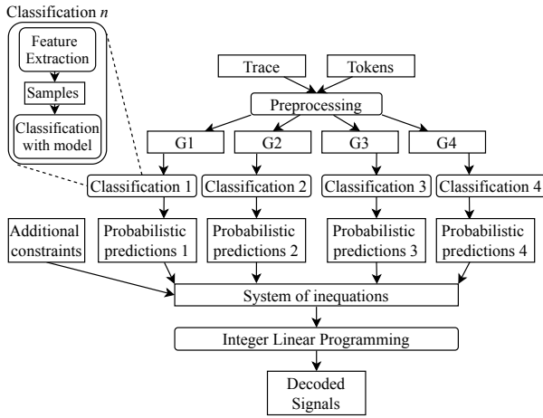
Figure 2. Pipeline of CSI.
