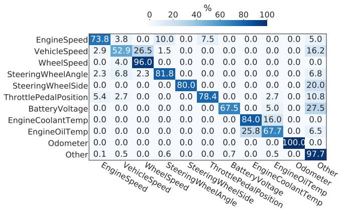
Figure 3. Confusion matrix of the predictions performed by CSI with MLP.
