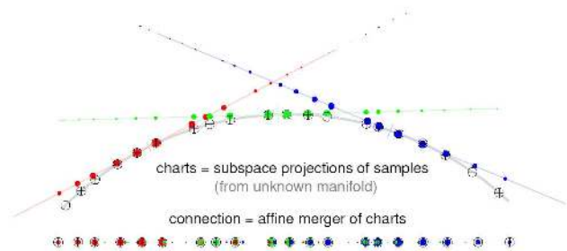
Figure 10: A simple charting example. Points ( \oplus ) sampled from an unknown manifold (gray curve) are projected onto three subspaces (red, green, and blue lines) and assigned a probability (indicated by size) according to their distance from the point where the chart touches the manifold. A minimal-distortion merger of these charts gives a flattening of the manifold in a lower dimensional space, where the mapped locations of points are the probability-weighted combinations of their chart-specific locations.
