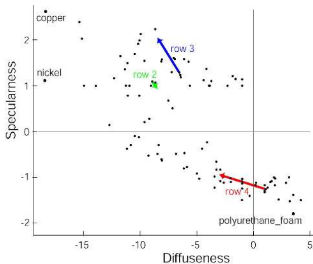
Figure 12: Diffuseness trait vs specularness trait. Observe that the diffuseness and specularness traits exhibit a weak inverse correlation. The green, blue, and red vectors denote projections of the BRDF interpolations shown in the second, third, and fourth rows of Figure 16 respectively.
