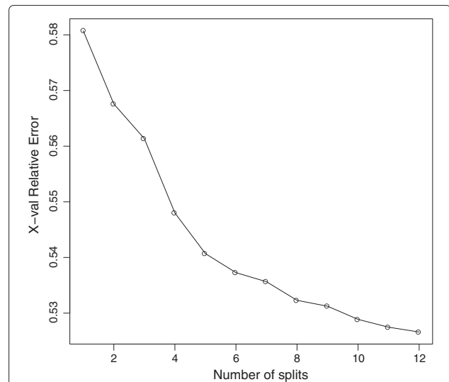
Figure 4 Reduction of the MSE according to the number of splits.
