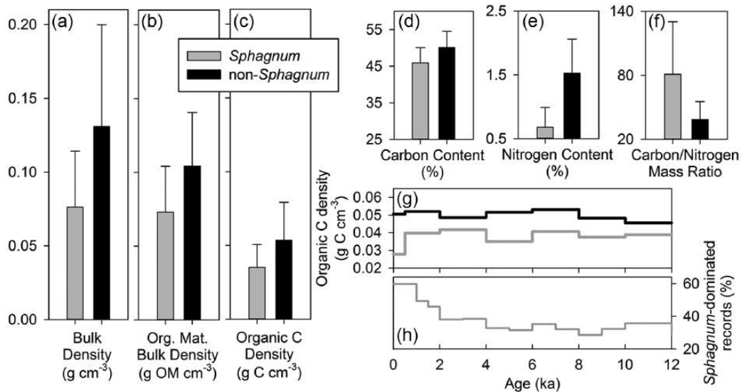
Figure 6. Main differences between Sphagnum and non- Sphagnum peat samples: (a) bulk density, (b) organic matter bulk density, (c) organic carbon bulk density, (d) carbon content, (e) nitrogen content, (f) carbon/nitrogen mass ratio, (g) temporal pattern of organic carbon bulk density, and (h) proportional change in the number of peat records that are Sphagnum -dominated, presented as a percentage of the total number of records.
