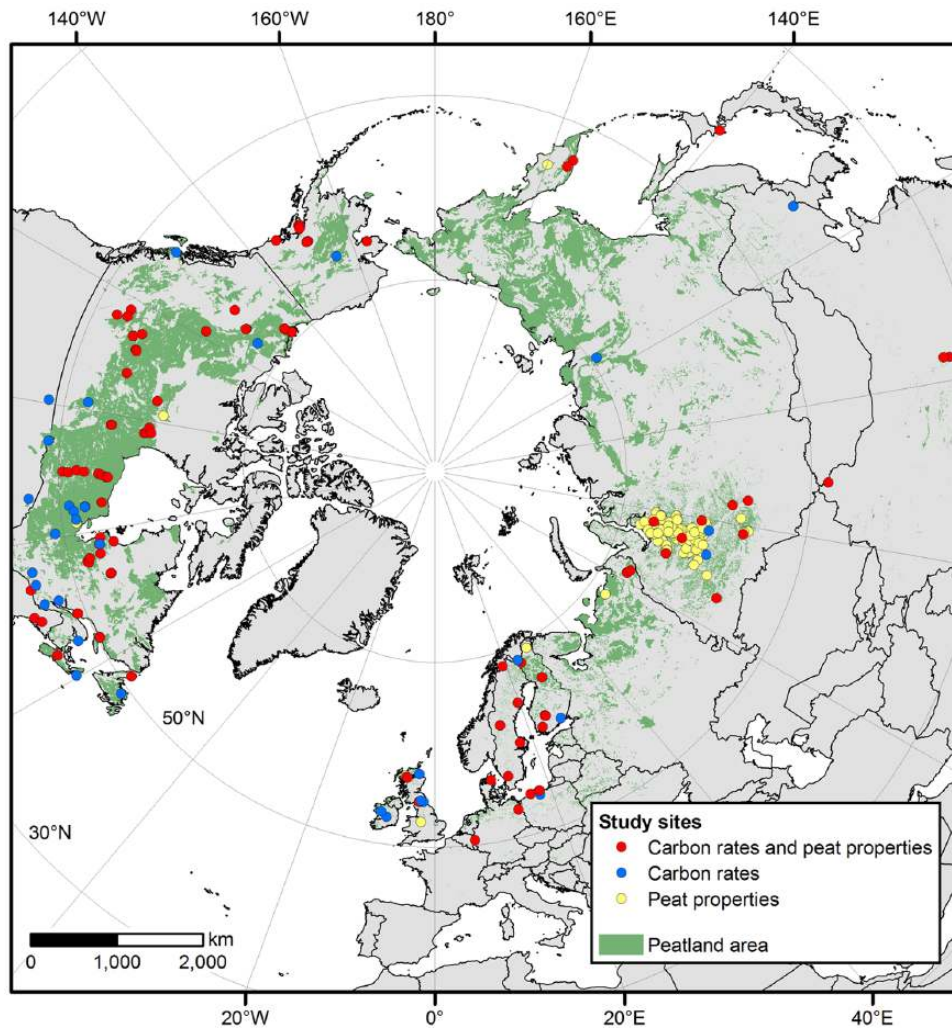
Figure 1. Location of study sites. Map showing the distribution of northern peatlands (green area from Yu et al., 2010) and peatland sites included in this study ( n = 215 sites, including 268 peat cores). Long-term rate of peat carbon accumulation was estimated from 127 sites (151 peat cores; red and blue dots). The yellow dots represent cores for which only peat properties (bulk density, organic matter content, etc.) were available and synthesized. Refer to Supplementary Table S1 (available online) for details.
