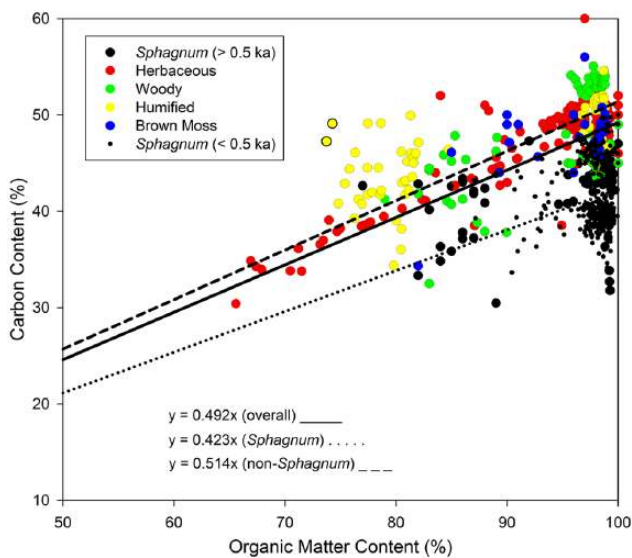
Figure 4. Relation between carbon content and organic matter content in northern peatlands. The slope of each regression line is used as a conversion factor for estimating carbon content from organic matter content.
