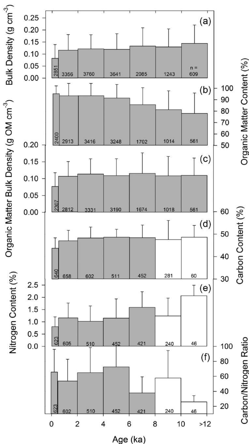
Figure 5. Temporal patterns of peat properties (mean, standard deviation, and number of samples): (a) bulk density, (b) organic matter content, (c) organic matter bulk density, (d) carbon content, (e) nitrogen content, and (f) carbon/nitrogen mass ratio. White bars represent values that were based on a limited number of samples and peat records.
