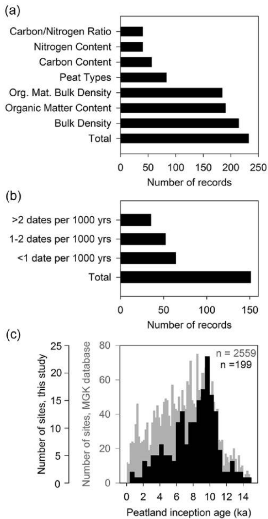
Figure 2. Overview of data availability. (a) Number of cores (total = 238) containing information on carbon/nitrogen ratio ( n = 40 ), nitrogen content ( n = 40 ), carbon content ( n = 56 ), peat types ( n = 83 ), organic matter bulk density ( n = 184 ), organic matter content ( n = 190 ), and bulk density ( n = 214 ). (b) Number of cores (total = 151) with a dating quality better than two dates per 1000 years ( n = 35 ), one to two dates per 1000 years ( n = 52 ), and less than one date per 1000 years ( n = 64 ). (c) Number of calibrated basal peat ages (median) in 500-year bins from the database ( n = 199 ) compared with all northern hemisphere basal peat ages (median) in 200-year bins ( n = 2559 , MGK data from Gorham et al., 2007; Korhola et al., 2010; MacDonald et al., 2006).
