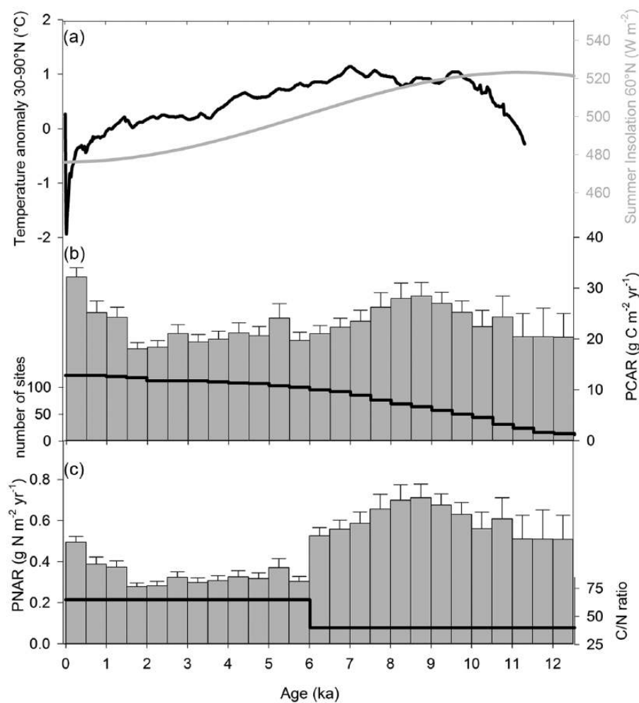
Figure 7. Long-term apparent rate of carbon and nitrogen accumulation from northern peatlands ( n = 127 sites). (a) Summer insolation at 60°N (data from Berger and Loutre, 1991) and temperature anomaly from an 11,300-year reconstruction for the northern region from 30° to 90°N (data from Marcott et al., 2013). Temperature anomaly was calculated based on the 1961–1990 temperature averages. (b) Mean peat carbon accumulation rates (PCAR) and standard error in 500-year bins. The number of sites per 500-year bins is also presented as step lines. (c) Mean peat nitrogen accumulation rates (PNAR) and standard error in 500-year bins. These values were obtained using different C/N values over time, as indicated by the line.
