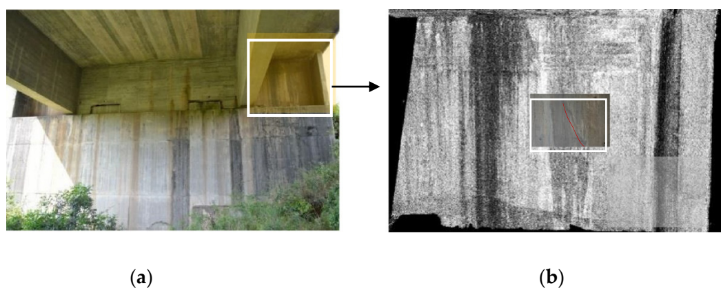
Figure 7. Crack characterization using integrated laser scanning and image processing: (a) identified critical region; (b) 3D model of critical region [47].
