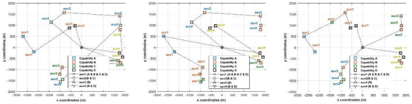
Figure 5: Goal allocation and task distribution using POPF (left), OPTIC (middle) and DHRHTA+TP (right). Plans are evaluated by simulation for a set of five heterogeneous AUVs. DHRHTA+TP reduces the complexity of the mission plan by considering the goal coordinates and capability requirements.
