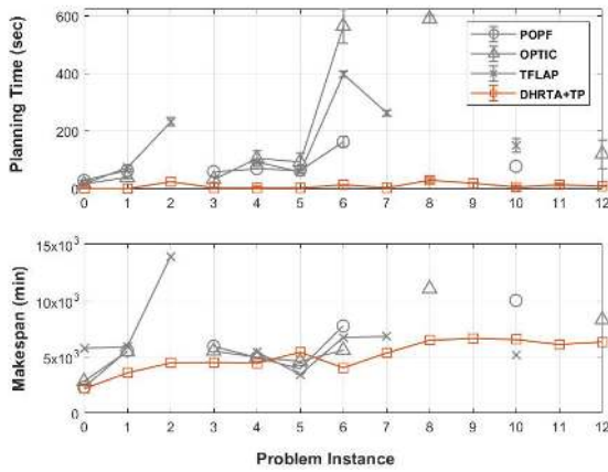
Figure 6: Planning time (top) and makespan (bottom) analysis for DHRHTA+TP and benchmark planners. DHRHTA improves temporal planning performance by reducing planning time, which improves the response capacity of the robotic system while keeping makespan at similar values compared with the solutions generated by the benchmark planners.
