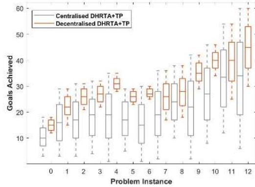
Figure 7: Number of goals achieved by DHRHTA+TP during mission execution, with task failure occurring at random times. Results are compared against a centralised planner.
