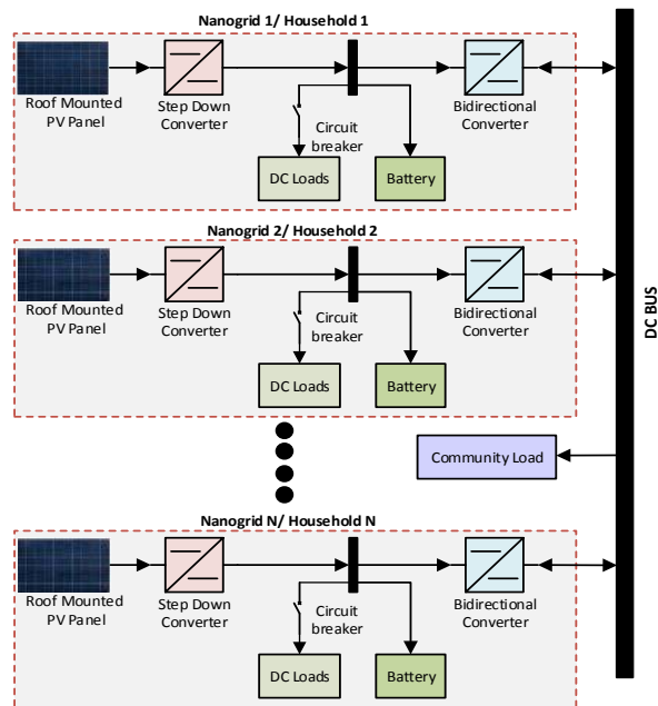
Fig. 1. A cluster of multiple nanogrids interconnected via DC bus formulating the DGDSA of PV/battery-based DC microgrid.
