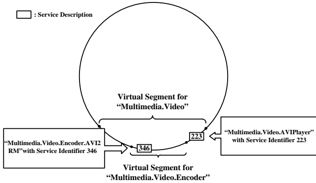
Fig. 2. Virtual segments for “Multimedia.Video” and “Multimedia.Video.Encoder”.
