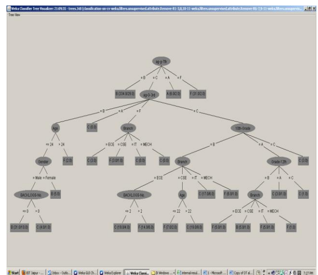
Fig 1: Decision Tree Construction
