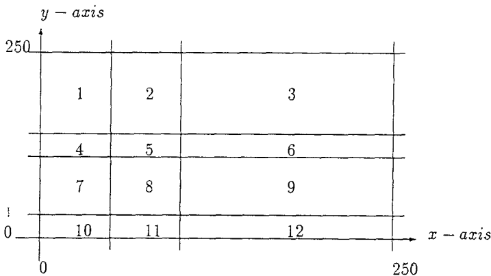
Fig. 1. Clustered problem m_1 = 2, m_2 = 3 .
