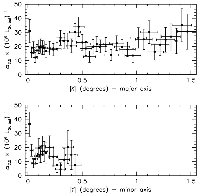
Figure 31. Variation of \alpha_{2.5} with distance along the major and minor axes. \alpha_{2.5} is estimated at positions along the two axes where Walterbos & Kennicutt (1987) listed a value for the surface brightness; the number density of PNe at each location is estimated from the number of PNe in a box whose dimensions are equal to the horizontal error bar.
