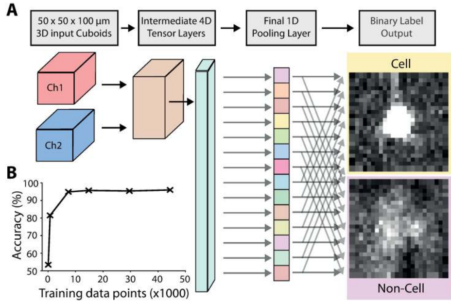
Fig 3. Cell classification. A: The input data to the modified ResNet are 3D image cuboids (50 μm x 50 μm x 100 μm) centered on each cell candidate. There are two cuboids, one from the primary signal channel, and one from the secondary autofluorescence channel. The data is then fed through the network, resulting in a binary label of cell or non-cell. During training the network “learns” to distinguish true cells, from other bright non-cellular objects. See S3 and S4 Figs for more details of the 3D ResNet architecture. B: Training the initial cell classification network: classification accuracy as a function of training data quantity.
