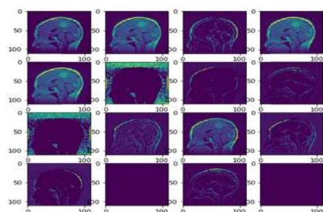
(a) FM-C1-DensNet
