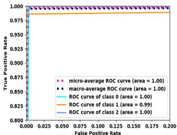
(b) combined_densnet_block
