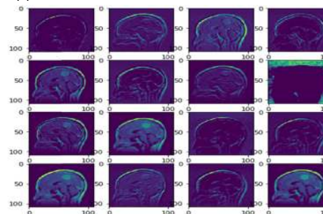
(b) FM-C1-Inception
