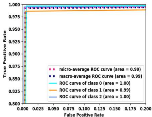
(a) combined_inception_block
