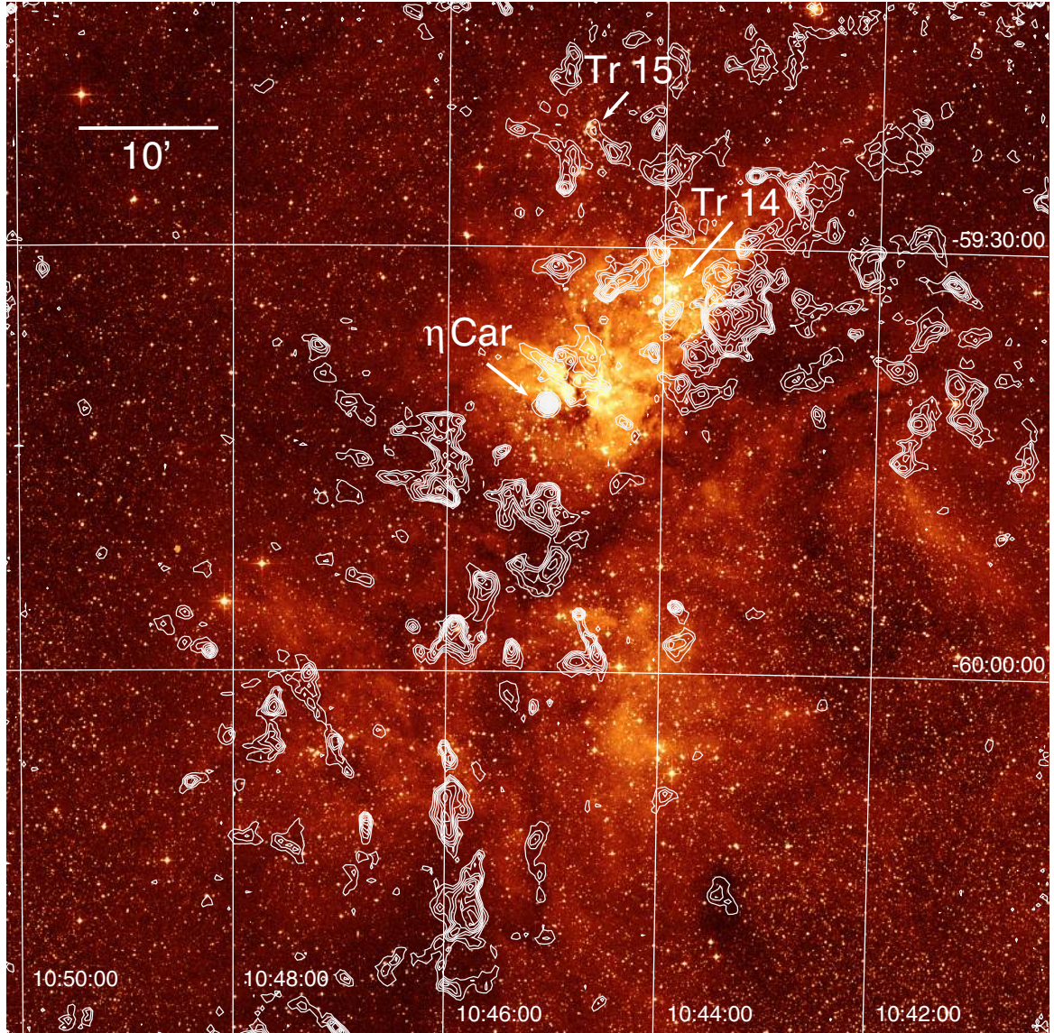
Fig. 2. False-color representation of the red optical Digitized Sky Survey image with contours of the LABOCA map overlaid. Here and (unless noted otherwise) in the following images, the first three contour levels are 0.06, 0.12, and 0.18 Jy/beam, while the further levels increase by a factor of \sqrt{2} . The grid shows the J2000 coordinates.
