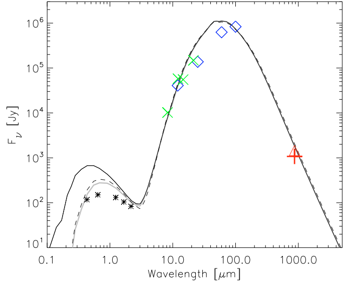
Fig. 9. Spectral energy distribution of the Carina Nebula complex. The diamonds and crosses show the mid- and far-infrared fluxes determined from the IRAS and MSX maps for the field of the LABOCA map. The cross with the upward triangle shows the total 870\ \mu\text{m} flux derived from our LABOCA map (excluding the emission from \eta Car and the Keyhole Nebula). The asterisks show the integrated optical and near-infrared fluxes of the known stellar members of Carina as identified in a deep Chandra X-ray survey (see Preibisch et al. 2011b). The solid line shows the spectral energy distribution resulting from our spherical cloud model of the CNC with a total gas + dust mass of 140\,000\ M_{\odot} ; the gray line shows the effect of adding 1 mag of visual foreground extinction to the spectrum. The dashed line is the model with a cloud mass of 280\,000\ M_{\odot} .
