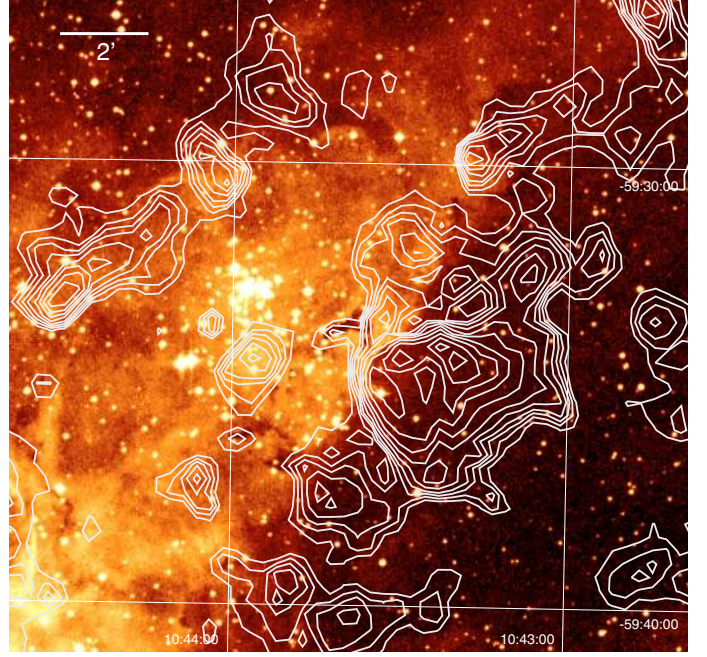
Fig. 4. False-color representation of the red DSS image for the region near Tr 14 with superposed contours of the LABOCA map.
