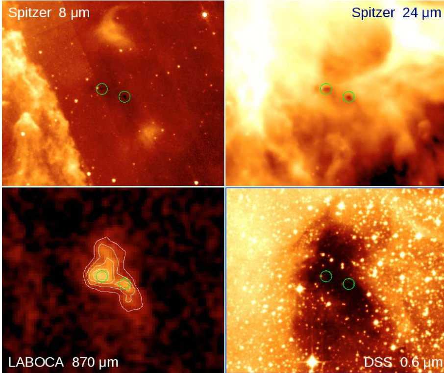
Fig. 7. False-color images of the region around the infrared dark cloud, seen in the Spitzer 8 \mu\text{m} IRAC map ( upper left ), the 24 \mu\text{m} MIPS map ( upper right ), the LABOCA map ( lower left ), and the optical DSS image ( lower right ). In each image, the field-of-view is \approx 8.2' \times 6.6' , north is up, east to the left. The contour levels superposed onto the LABOCA map are 0.06, 0.09, 0.12, and 0.15 Jy/beam. The two peaks are marked by green circles.
