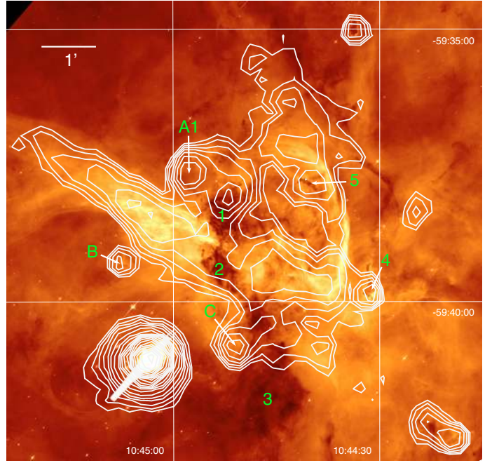
Fig. 3. False-color representation of the HST H\alpha image of \eta Car and the Keyhole Nebula with superposed contours of the LABOCA map. The numbers 1–5, A1, B, and C refer to the CO clumps in the Keyhole Nebula defined in Cox & Bronfman (1995). The contour levels in this image start at 0.06 Jy/beam and increase on a logarithmic scale by factors of 1.364 (i.e. 0.135 dex).
