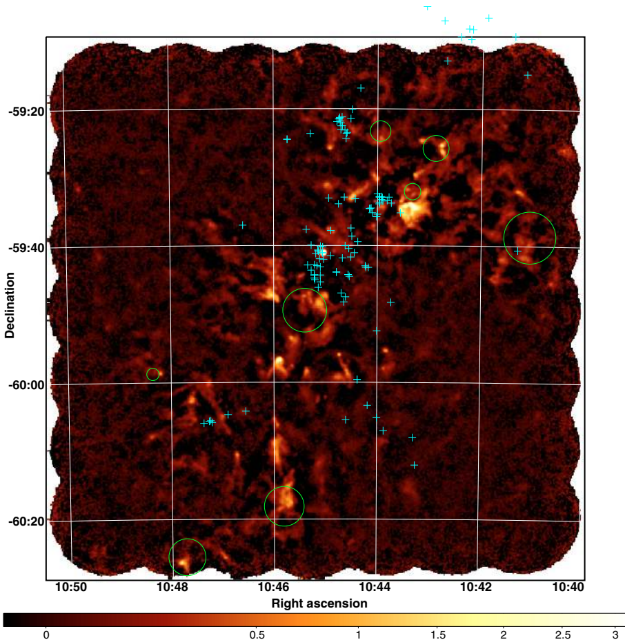
Fig. 1. False-color representation of the wide-field LABOCA map of the Carina Nebula complex. The cyan crosses mark the positions of the massive (O- and early B-type) stellar members of the Carina Nebula from Smith (2006) , the green circles mark the locations and radii of the dense C^{18}O clumps detected by Yonekura et al. (2005) in this area. The field-of-view is \approx 1.3^\circ \times 1.3^\circ , corresponding to a size of \approx 52 \times 52 pc at the distance of the complex; the grid shows the J2000 coordinates. The units of the scale bar at the bottom are Jy/beam.
