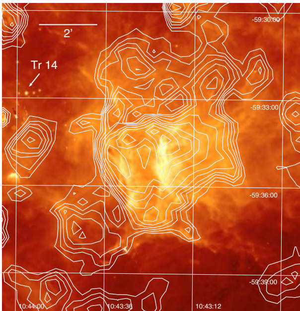
Fig. 8. False-color representation of the 8.0 \mu\text{m} Spitzer image of the cloud west of Tr 14 with superposed contours of the LABOCA map.
