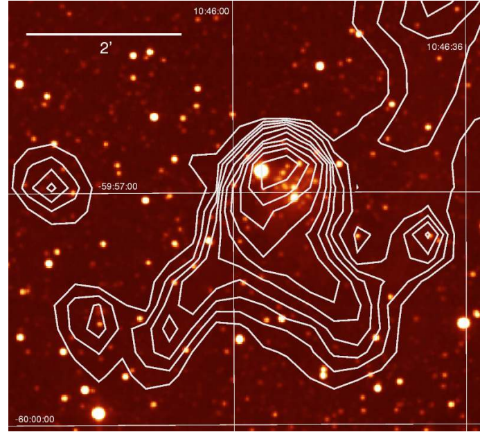
Fig. 5. False-color representation of the 2MASS K -band image of the area around the Treasure Chest Cluster (located at RA (J2000) = 10^{\text{h}}45^{\text{m}}54^{\text{s}} , Dec = -59^{\circ}56'50'' ) with superposed contours of the LABOCA map.
