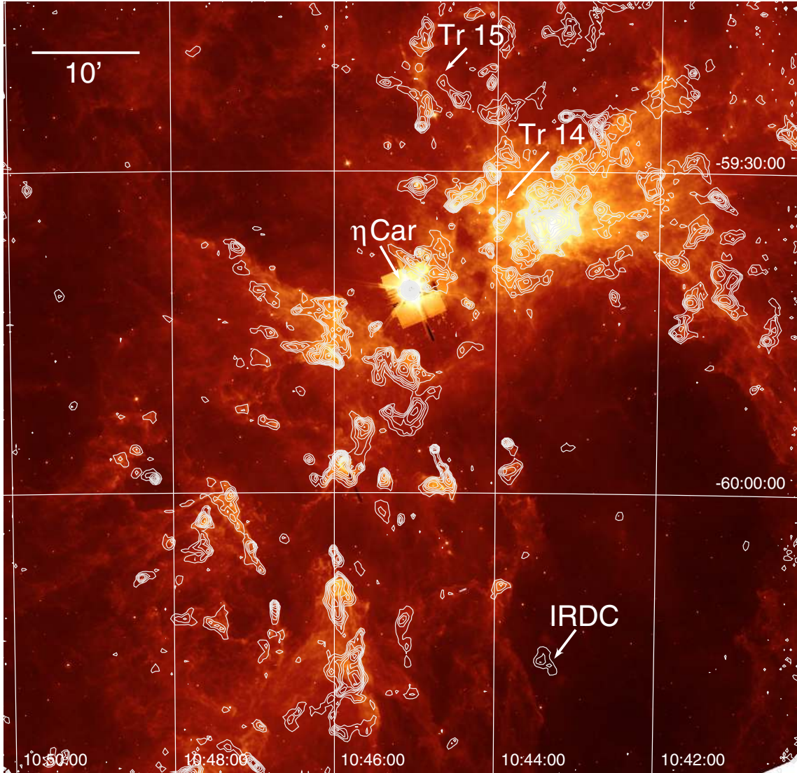
Fig. 6. False-color representation of the 8.0\ \mu\text{m} Spitzer image with superposed contours of the LABOCA map. In the area within a few arcminutes from \eta Car the very bright infrared emission caused strong artifacts in the Spitzer image. A grid of J2000 coordinates is shown.
