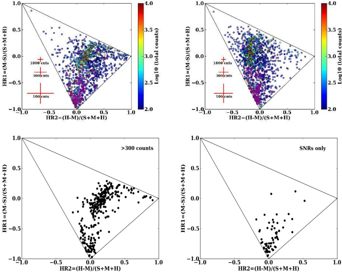
FIG. 6.— Top left : Hardness ratios from fluxes in the 0.2-1.0, 1.0-2.0, and 2.0-4.5 keV bands of all unflagged, s-flagged, t-flagged, or matched to T11 sources with >50 source counts in Table 3. These fluxes use the ECFs in Table 2, which assume a power-law spectrum with index 1.7 and absorption 6 \times 10^{20} \text{ cm}^{-2} . The 0.2-1.0 keV fluxes are the sum of the 0.2-0.5 keV and 0.5-1.0 keV fluxes in Table 3. Fluxes are used for the HRs in this plot to make our catalog easier to compare with those measured with other X-ray observatories. H = 2.0\text{-}4.5 keV flux; M = 1.0\text{-}2.0 keV flux; S = 0.2\text{-}1.0 keV flux. Upper limits were applied in bands with 0 counts to calculate ratios, so that no sources fall outside of the area allowed by positive flux measurements. Blue to red colors show the number of counts in the measurement. Known SNRs are highlighted with purple circles. Approximate uncertainties for a range of total counts are shown with the red crosses. Top right : Same as top-left, but ratios were calculated from count rates. Bottom left : Same as top-left, but without color-coding and showing only sources with >300 source counts in our catalog are shown. The sequence from the soft thermal sources to the hard, absorbed power-law sources is much clearer. Bottom right : Same as top-left, but without color-coding and showing only known SNRs, which have a markedly softer distribution than the full source population.
