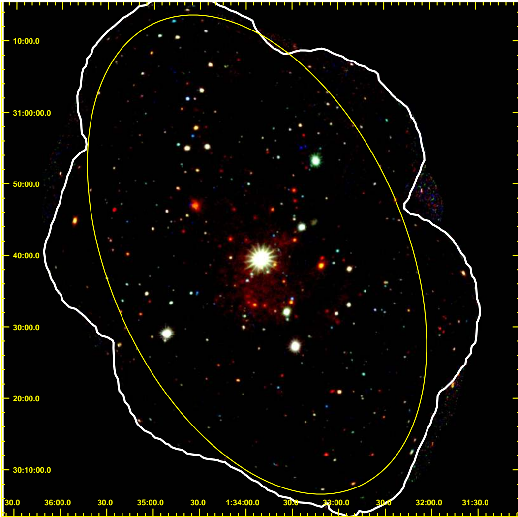
FIG. 1.— Our color composite image of M33 from all of the observations listed in Table 1. Yellow ellipse marks the M33 D_{25} region, and the white contour marks the area with at least 40 ks of exposure. Red is 0.2-0.5 keV. Green is 1-2 keV, and Blue is 2-4.5 keV.
