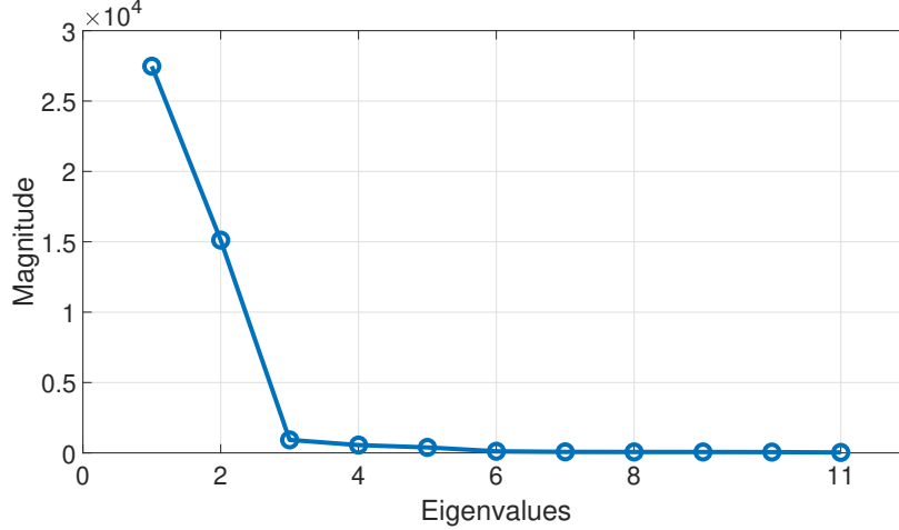
Figure 2. The 10 largest eigenvalues for the Hessian in Venice problem.
