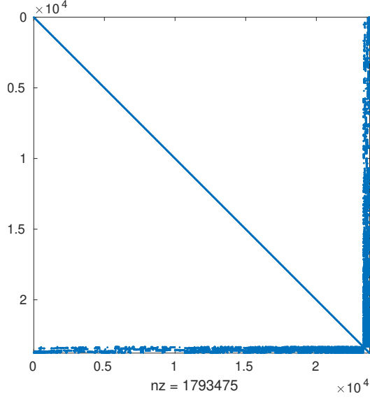
Figure 1. The Hessian is of size 23769 \times 23769 and has 1793475 non zero entries. For this dataset, number of camera parameters, c = 9 . The Ladybug-49 problem has 49 cameras and 7776 3D features. Thus, the camera submatrix has (9 \times 49 =) 441 rows (and columns), and the structure submatrix has (3 \times 7776 =) 23328 rows (and columns). Thus, the Hessian has (23328 + 441 =) 23769 rows as well as columns.
