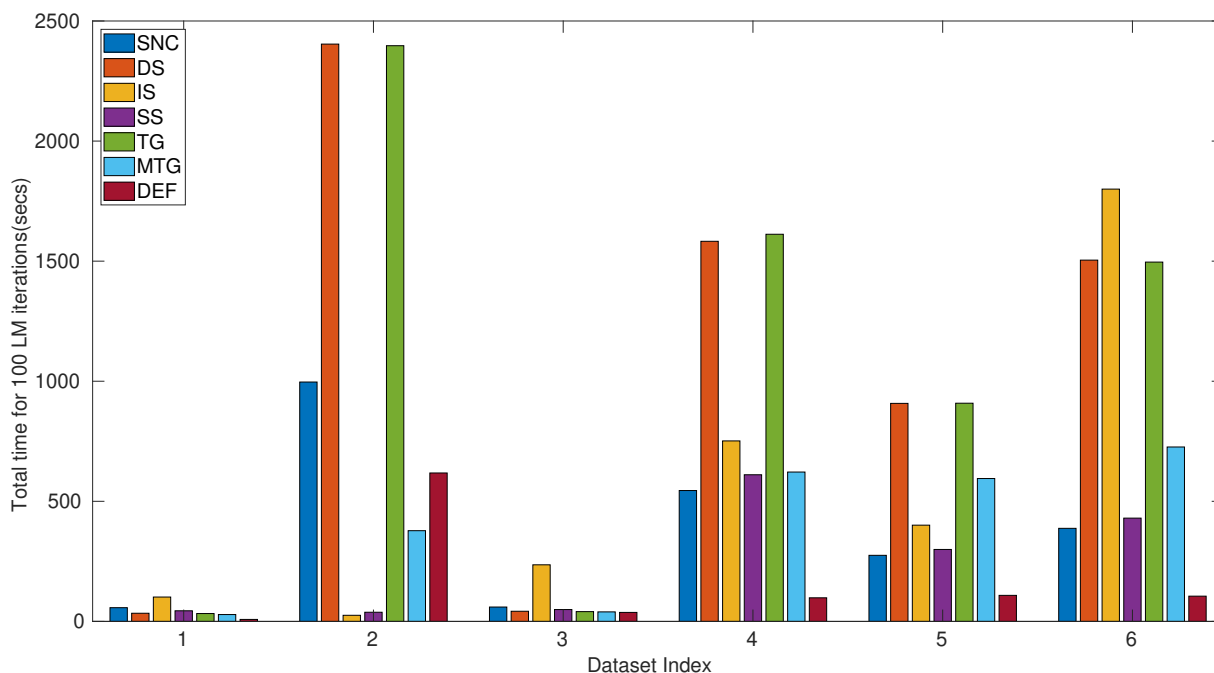
Figure 4. Bar plot of time comparisons for various solvers. Note that for dataset 2, the LM iterations do not converge using DEF solver, and for dataset 6, the LM iterations do converge using IS solver. Here, SNC stands for Sparse Normal Cholesky, DS stands for Dense Schur, IS stands for Iterative Schur, SS stands for Sparse Schur, TG stands for Two Grid [12], MTG stands for Modified Two Grid, and DEF stands for the Deflation preconditioner proposed in this work.
