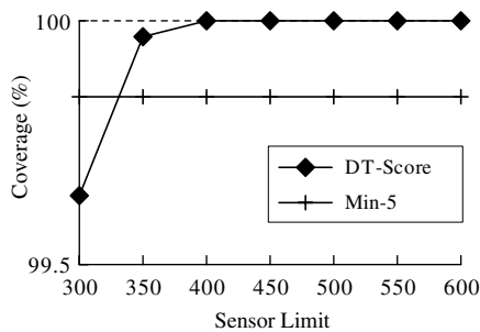
(b) Compare DT-Score and Min-5
