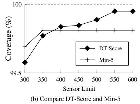
Fig. 17. Results of test case 4.
