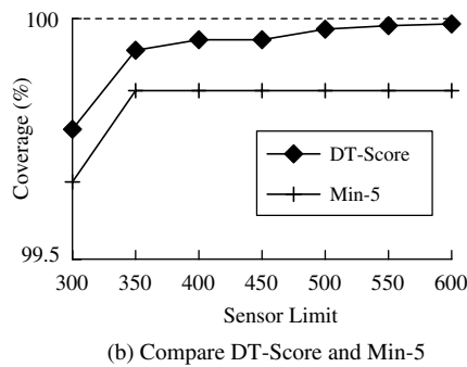
Fig. 16. Results of test case 3.
