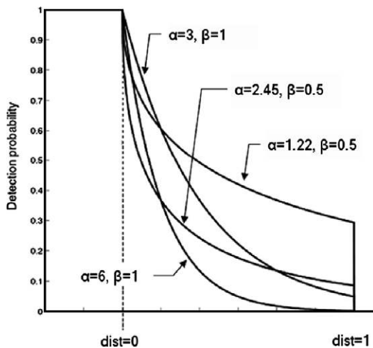
Fig. 3. The probabilistic sensor detection model.
