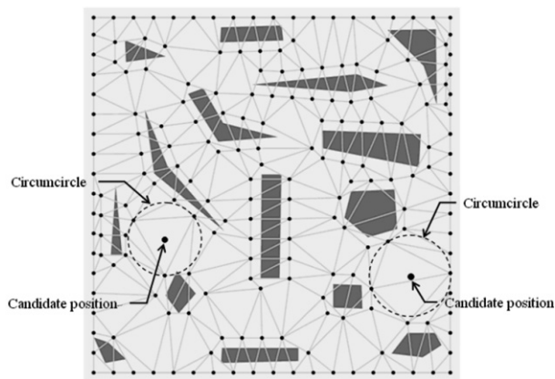
Fig. 8. The Delaunay Triangulation of given sensors.
