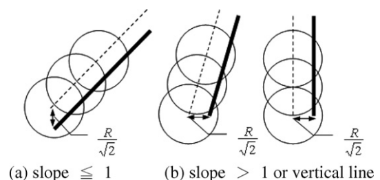
Fig. 6. Offset under different slope.
