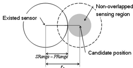
Fig. 9. Overlapping with other sensor.
