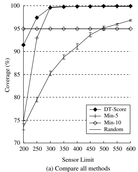
(a) Compare all methods
