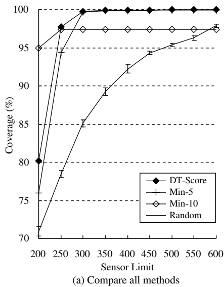
(a) Compare all methods
