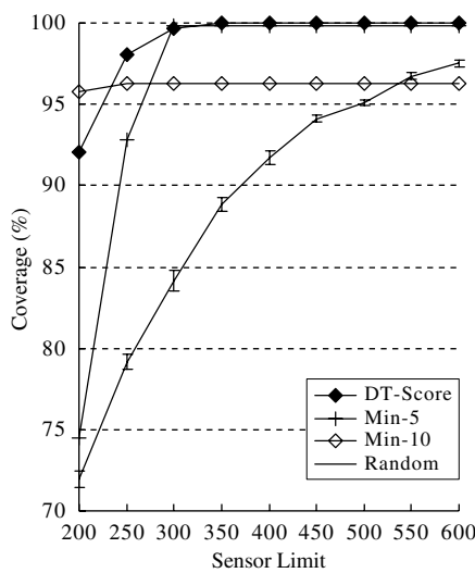
(a) Compare all methods
