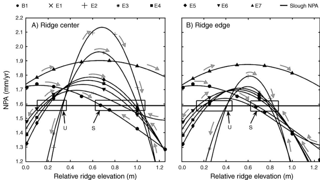
FIG. 7. Net peat accretion (NPA) vs. ridge elevation at (A) ridge center and (B) ridge edge for different possible depth/redox potential relationships (Appendix E) for the oligotrophic Everglades (Table 3). Data points represent individual simulation results, grouped by their association with a unique set of parameter values. Smooth curves are cubic least-squares regressions for each set of simulation results. The relative ridge elevation for each point is the elevation at which the simulation was initialized, and NPA was determined from the second year of simulation. Note that curves do not directly show temporal evolution of ridges, but temporal evolution is implied by the gray arrows indicating the direction of ridge growth (relative to slough growth) over time. Boxes indicate the loci where the family of curves cross the mean rate of NPA in sloughs, at which the rate of NPA on ridges and sloughs is equivalent. The box labeled “U” corresponds to the family of unstable equilibrium points, which physically correspond to required initiation heights for ridge growth under this differential peat accretion feedback mechanism. The box labeled “S” corresponds to the family of stable equilibrium points, which physically correspond to equilibrium ridge heights. Ridges initiated anywhere to the left of “U” approach the stable equilibrium height “S” with respect to slough bottoms, whereas ridges initiated to the left of “U” subside and become indistinguishable from the slough.
