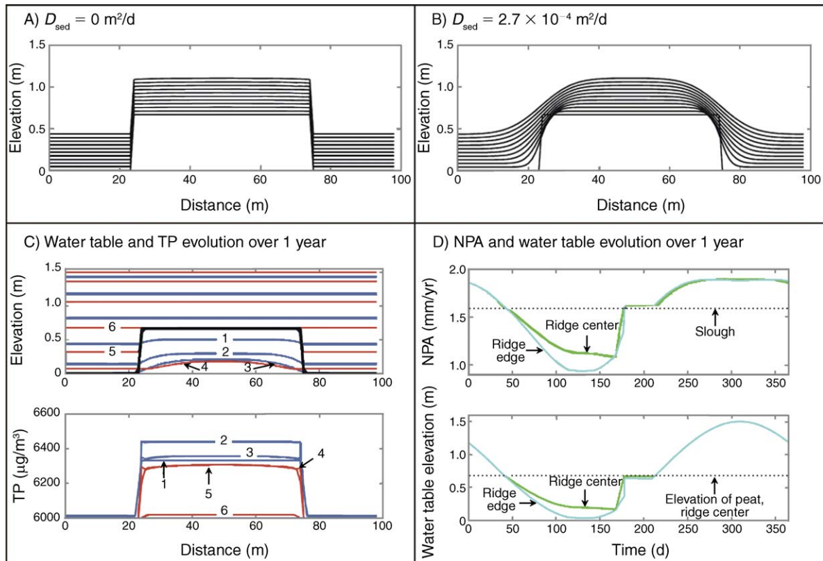
FIG. 6. PeatAccrete 1.0 simulation results for depth/redox case B1 (Appendix E). In (A) and (B), peat surface topography is depicted for 100 000 days ( \sim 274 years) of simulation. Peat surface elevation is plotted against cross-sectional distance for the initial time step and 10 intermediate time steps, evenly spaced in time (every 10 000 days throughout the simulation). Plot (A) shows the evolution of state variables when lateral erosion of soil has been turned off. In plot (B), erosion is turned on, with the soil diffusivity coefficient ( D_{\text{sed}} ) set equal to the default value in Appendix B. Plots (C) and (D) show the evolution of total phosphorus (TP), water table, and net peat accretion (NPA) over the course of one year for the nonzero D_{\text{sed}} case, with (C) depicting TP and water table values along a cross-sectional transect for 12 evenly spaced times throughout the year (red and blue lines distinguish between periods of rising water level and periods of falling water level, respectively, while the black line shows the ridge topography) and (D) depicting the continuous evolution of NPA and water table at two points on the ridge in response to seasonal changes in evapotranspiration and precipitation. In (C), not all TP profiles are apparent, as profiles are flat, featureless, and equivalent to the background concentration of TP when water covers ridge surfaces. During the dry season, when ridges are exposed, an evaporative concentration signature is apparent in the elevated TP concentrations. Apparent TP concentration profiles and their corresponding water table are numbered accordingly.
