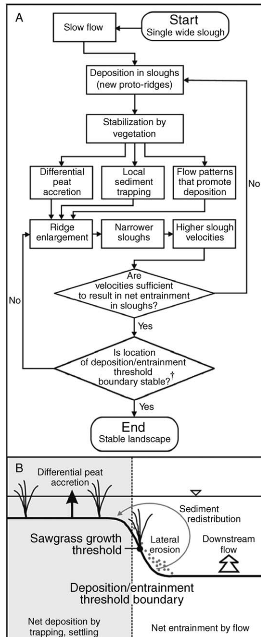
FIG. 4. (A) Flow chart and schematic diagram of proposed RSL evolution, beginning with regional slough conditions (Bernhardt et al. 2004) and ending with a stable, regularly patterned landscape. In the equilibrium landscape, the characteristic ridge width and spacing reflect the morphology in which the capacity for sloughs to transport sediment and organic matter downstream and to ridges balances in situ organic matter production and gravitational erosion so that the NPA within sloughs is equivalent to that on ridges. The question followed by a dagger ( \dagger ) symbol asks whether the boundary between net entrainment of bed sediment and net deposition of bed sediment moves slough-ward over time. (B) Diagram clarifying concepts outlined in (A), providing more detailed insight into the processes governing ridge width and spacing at a transition region between ridge and slough.
