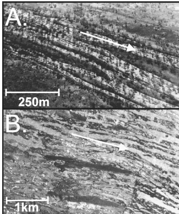
FIG. 3. Comparison between the geomorphology of the anabranching Marshall River, Australia, and the Everglades RSL, south Florida. Arrows indicate direction of flow. (A) An oblique aerial view of the anabranching Marshall River (image from Tooth and Nanson [2000]). (B) Satellite image of the RSL from Science Coordination Team (2003). Light features are ridges, and dark features are sloughs. The very dark feature at the center of the image is a tree island. Panel (A) is reproduced with permission from John Wiley and Sons.
