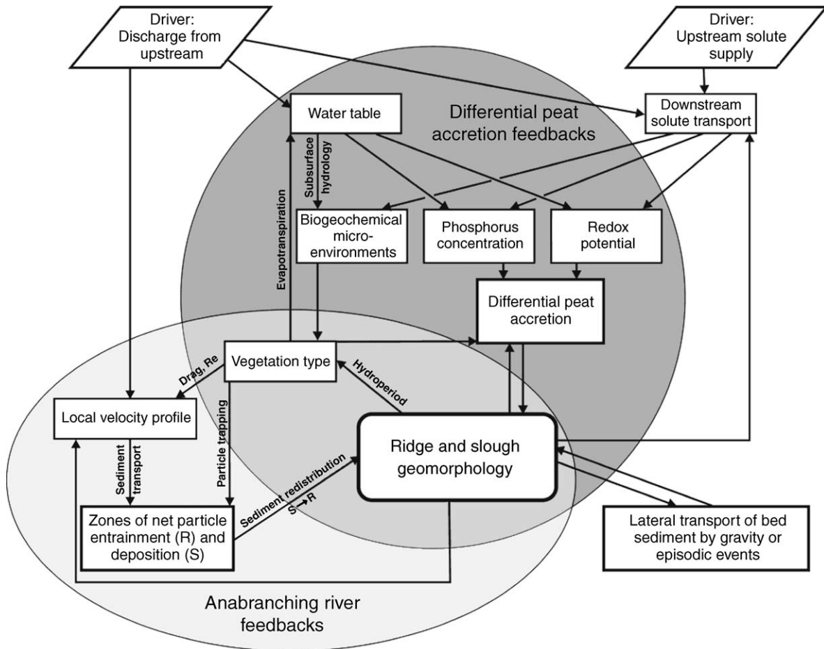
FIG. 2. Proposed conceptual model of the feedback mechanisms and processes governing Everglades ridge and slough landscape (RSL) morphology. The two major classes of feedback mechanisms (differential peat accretion and anabranching river feedbacks) are delineated with shaded ellipses. Reynolds number is abbreviated “Re.”
