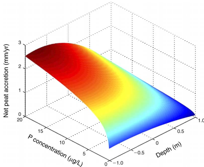
FIG. 5. Response surface of simulated net peat accretion (NPA) to total phosphorus (TP) concentration and depth. Negative depths refer to cases in which a free-water surface is present. Since depth controls redox potential in the oligotrophic Everglades (Appendix A; Kludze and DeLaune 1996), the depicted function may also be considered proportional to the relationship between NPA, TP, and redox potential ( E_h ), with E_h decreasing along the depth axis. The color of the response surface emphasizes net peat accretion rate values, with warmer colors corresponding to high net peat accretion rates and cooler colors corresponding to low net peat accretion rates.
