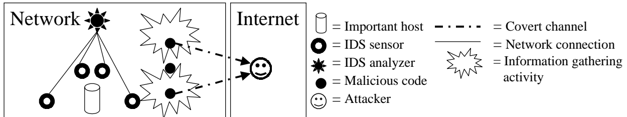
Figure 5.2: Malicious code gathers and reports information about the location of IDSs and important servers to the attacker
