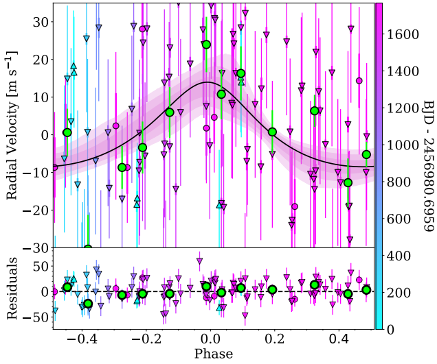
Figure 8. HD 18599 RVs folded at 4.137437 days. The black line represents the best fitting model while the purple shaded regions show the 1, 2 and 3 \sigma confidence regions of the model. The lower panel shows the residuals of the fit. Circles are HARPS_pre data, upside down triangles show HARPS_post data and upright triangles show the FEROS data. Green points show the data binned to 10 points in phase space. The colorbar encodes the observing time of each observation.
