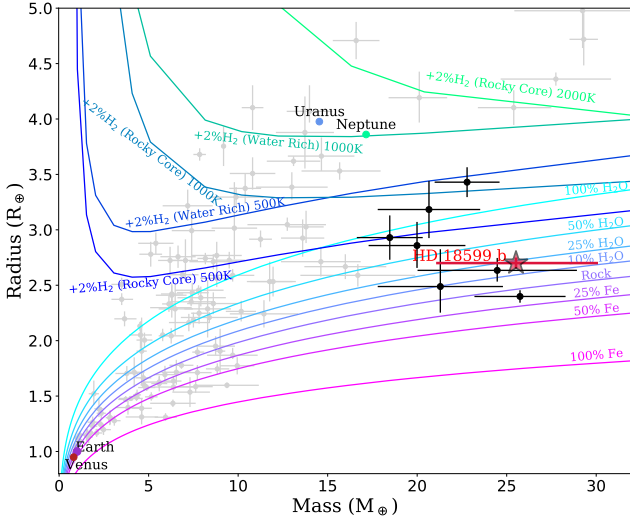
Figure 12. Mass-radius diagram for planets with masses and radii measured with a precision better than 20% (gray circles) in the range R_p < 5 R_\oplus and M_p < 30 M_\oplus , retrieved from the transiting exoplanets catalog TEPcat (Southworth 2011). Black points show relevant discoveries. HD 18599 b is shown with a red star. Solid, colored lines show different bi-layer composition models from Zeng et al. (2016), ranging from 100% iron core planet to 100% H_2O planet. Also five two-layer models from Zeng et al. (2019) are shown for 2% H_2 envelopes at different temperatures and core compositions.
