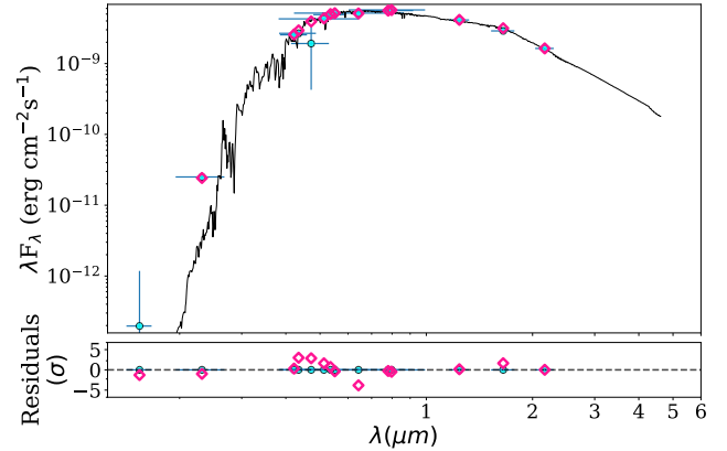
Figure 1. The best fitting Castelli & Kurucz SED (black line) for HD 18599 based on the photometric data (cyan points) presented in Table 3 is shown in the top panel. Horizontal errorbars show the bandpass width. The pink diamonds show the synthetic magnitudes at the wavelengths of the photometric data. The lower panel shows the residuals to the best fit model.
