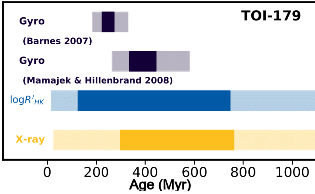
Figure 2. Different age estimates for HD 18599 using various methods.
