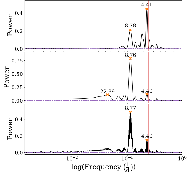
Figure 4. From top to bottom: the GLS periodogram for the TESS light curves from sectors 2 and 3 (top), sector 29 and 30 (middle), and the three sectors combined (bottom). The orange crosses show the most significant peaks with their respective periods labeled on top. The vertical red line marks the 4.1375-day planet candidate from the TESS data. The dashed horizontal line are the false alarm probabilities for 0.1, 5 and 10%, they turn out to be superimposed.
