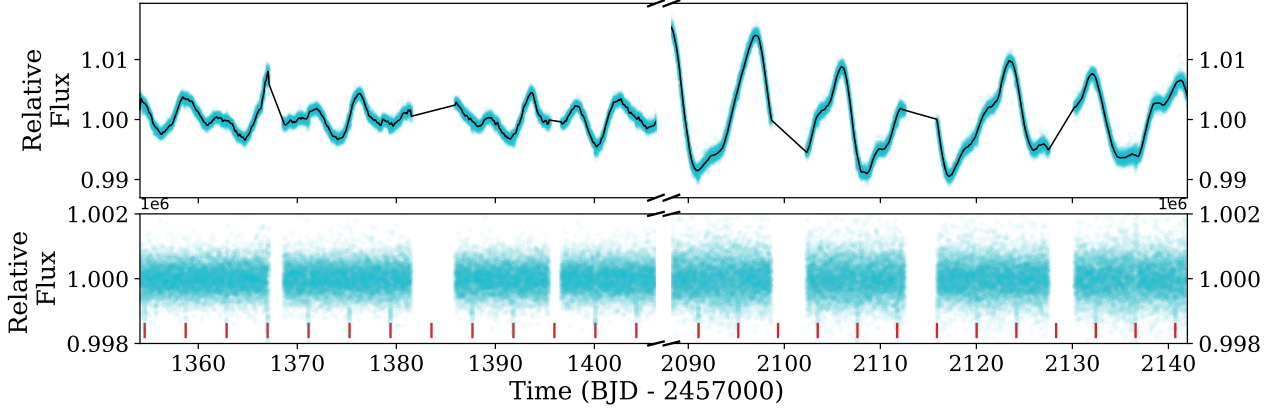
Figure 5. The normalized TESS light curve including data from the three sectors, with the best fitting SHO kernel GP (black line). The bottom panel shows the detrended light curve in ppm. The vertical red lines show the transit features.
