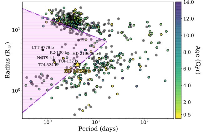
Figure 11. Period-radius diagram for planets with radii measured to a precision better than 5%. Relevant discoveries are named, and HD 18599 is shown with a big yellow star at the edge of the desert. The pink shaded area shows the Neptune desert, with the edges defined by Mazeh et al. (2016) . The colours show the ages of the systems and black shows systems without an estimated age. We note that ages have not all been measured in an uniform way.
