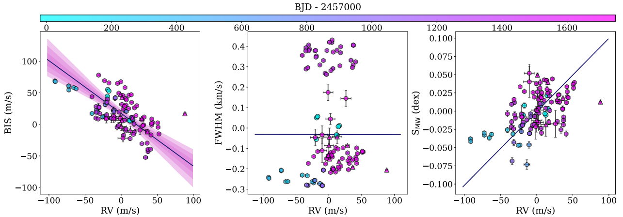
Figure 6. From left to right: The bisector velocity span with 1, 2 and 3 sigma confidence regions, FWHM, and S-index correlation with the RVs after subtracting their respective mean values. HARPS_pre, HARPS_post, and FEROS are denoted by circles, hexagons and triangles respectively. Each observation is color coded by its BJD timestamp. In all cases the blue line corresponds to the best fitting linear model. Confidence regions were not added for the FWHM and S index panels due to them being unconstrained.
