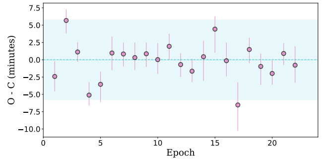
Figure 10. Observed minus computed mid-transit times for HD 18599b. The residuals (TTV) are shown considering the proposed ephemerides. The dashed cyan line shows zero variation and the shaded cyan region shows the 1 \sigma uncertainties on the linear ephemeris from EMPEROR. The plot shows no significant variation as all observations are within 1 \sigma of the best fitting ephemerides.
