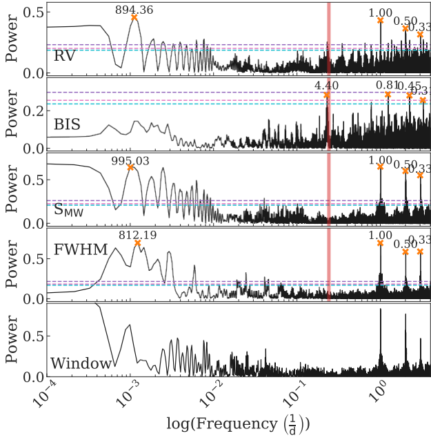
Figure 7. From top to bottom: the GLS periodogram for the RVs and activity indices from HARPS and FEROS: BIS, S-index, and CCF FWHM. The bottom panel shows the window function. Horizontal lines from top to bottom are the 0.1, 5 and 10% false alarm probabilities. The vertical red line marks the 4.1375-day planet candidate signal from the TESS data. The orange crosses show the most relevant peaks with their values in period written above them.
