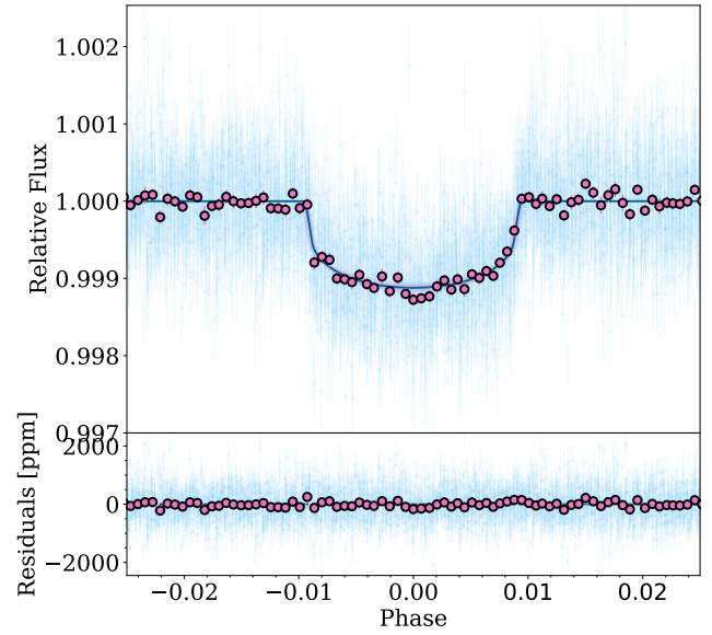
Figure 9. TESS light curve folded at 4.137437 days in light blue points with pink points showing the light curve binned to 50 points in phase space. The dark blue line represents the best fitting model and the pink shaded regions show the 1, 2 and 3 \sigma confidence regions of the model. The lower panel shows the residuals of the fit in ppm.
