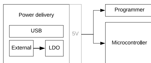
Figure 1. Arduino Uno power flow: power delivery either through USB or an external 12 V power supply, converted to a 5 V power rail powering both the always-on programmer and microcontroller.
