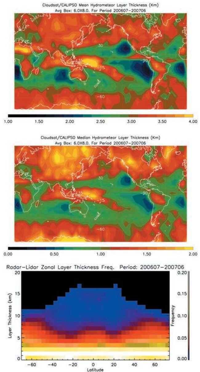
Figure 16. Hydrometeor (top) mean and (middle) median layer thickness and (bottom) the zonal layer thickness frequency distribution of all layers observed from July 2006 through June 2007 in 6 \times 8^\circ latitude-longitude averaging regions.
