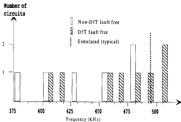
Fig. 16 - Capture range measurements on all functional samples of both the fault free PLL and PLL circuits with DfT
