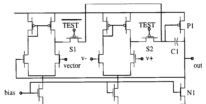
Fig. 5. Basic swap-amp structure
