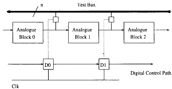
Fig. 3. Direct Drive into an Internal Circuit Node
