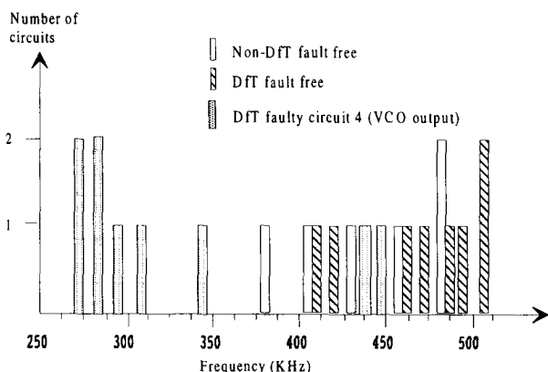
Fig 17 - Capture range for the DfT, non-DfT and faulty (circuit 4) versions of the PLL for all working samples
