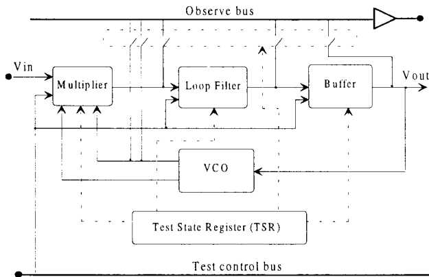
Fig. 9 PLL structure with DfT control
