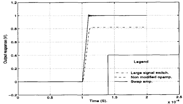
Fig. 7 HSPICE results for the circuits in Fig. 6
