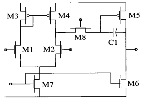
Fig. 4. The insertion of the switch M8 in the small signal path reduces the impact on circuit performance
