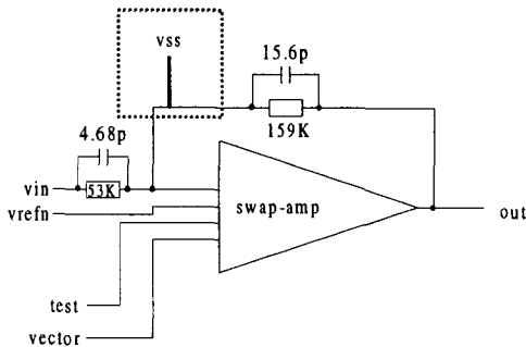
Fig. 12. S-A-0 short in feedback loop (circuit 3)
