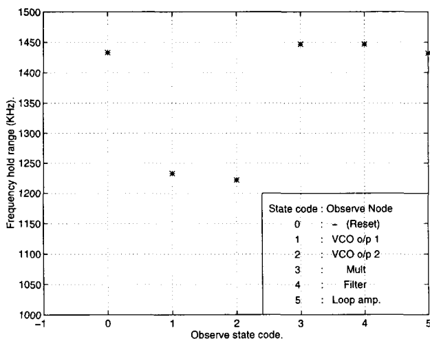
Fig 20 - Effect on the hold range of switching observability
