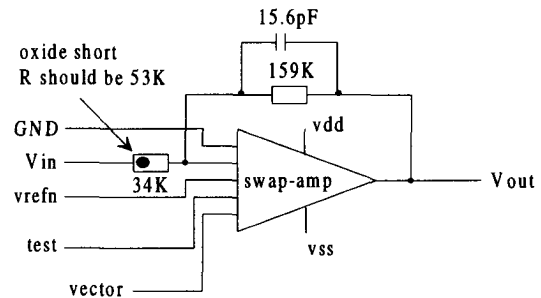
Fig. 14. Resistor snake shorted using a via to simulate gate oxide short in the loop filter block - (circuit 5)
