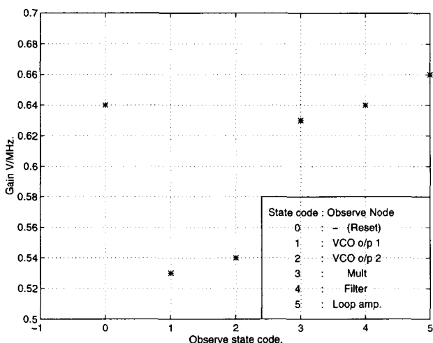
Fig 19 - Effect on the PLL gain of switching observability structures onto the test bus
