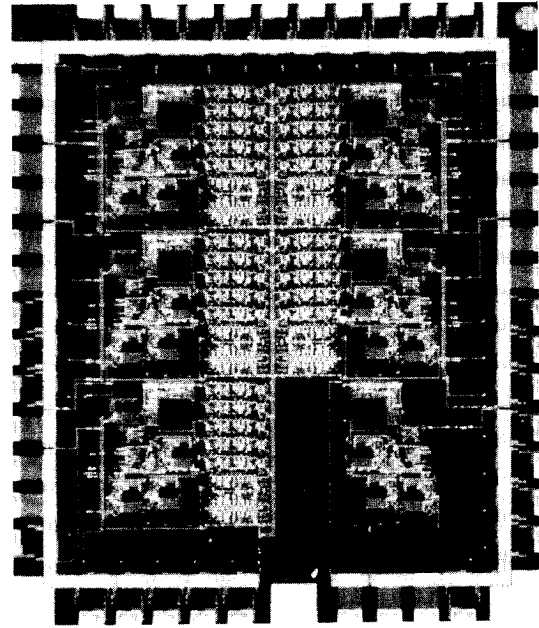
Fig 10. Test chip containing both faulty and fault free PLL circuits, with and without the DfT structures
