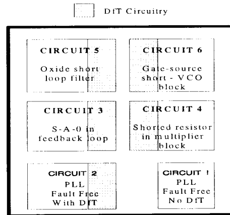
Fig 11. Floorplan of the test chip
