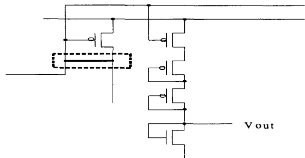
Fig. 15 - Gate-drain short in the VCO block.
