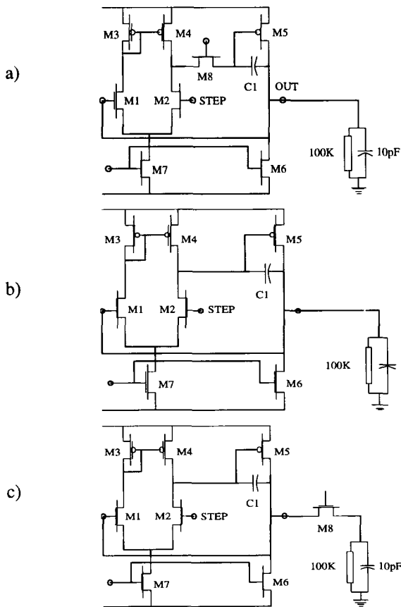
Fig. 6. Versions of the op-amp to be analysed. version (a) has the switch inserted in the small signal path, (b) no switch inserted (c) switch inserted in the large signal path
