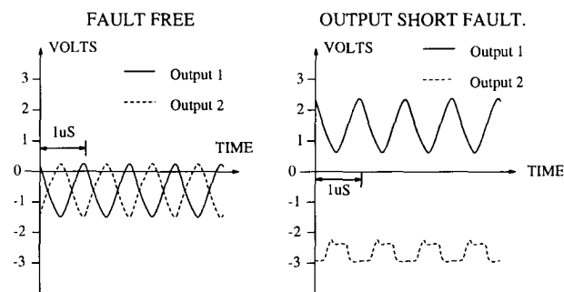
Fig 18 - a) fault free output from VCO output node and b) -VCO output response of faulty PLL version 2, IC number 7,- both measurements using the observe DfT feature
