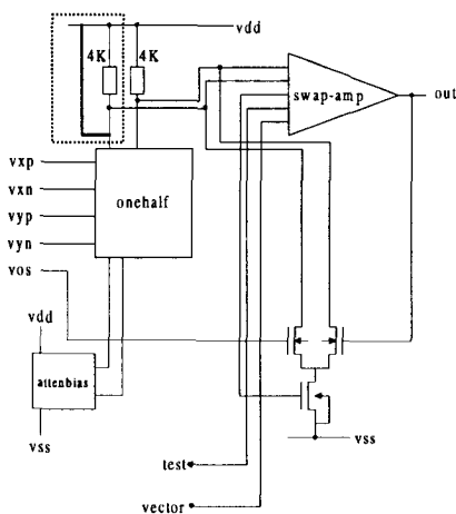
Fig. 13. Resistor shorted in 4 quadrant multiplier (circuit 4)
