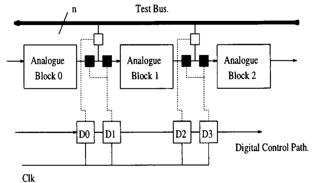
Fig. 2. DfT Strategy using switches between circuit blocks
