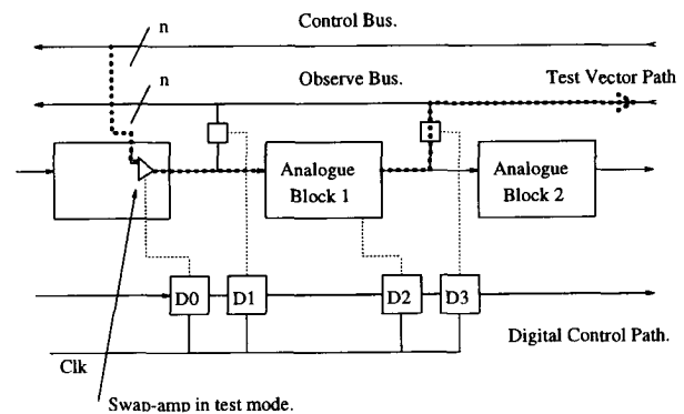
Fig 8.-The DfT strategy showing both access and observability features
