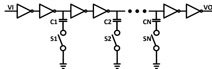
Figure 9. Schematic of variable delay cell.
