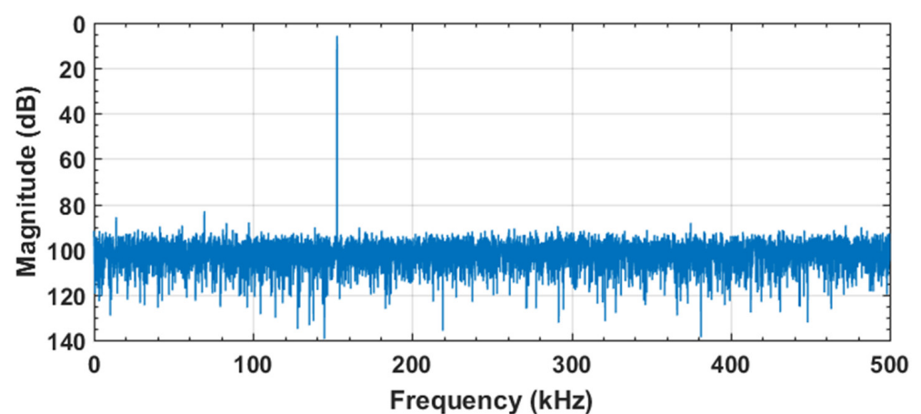
Figure 4. Dynamic performance of proposed switching with 1% unit capacitor mismatch.
