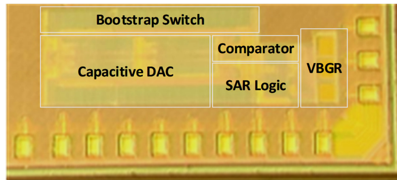
Figure 13. Die photograph of the asynchronous SAR ADC with VBGR.
