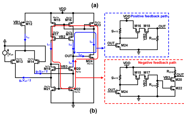
Figure 11. (a) Detailed schematic of the proposed error amplifier based bandgap reference voltage generator; (b) Proposed folded-Cascode error amplifier with intentional positive and negative feedback loop.
