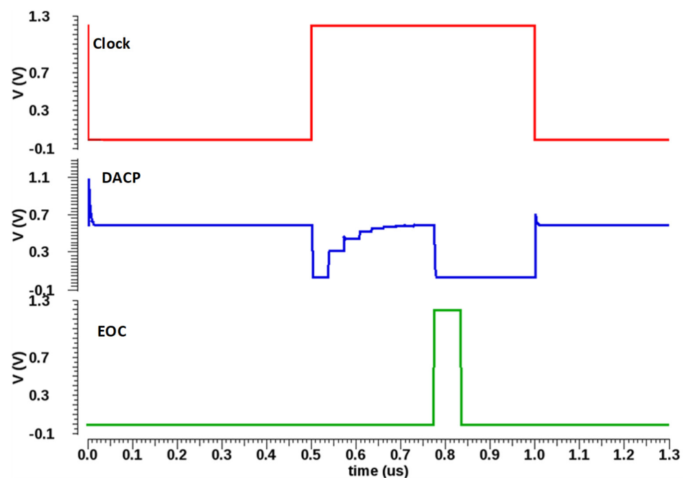
Figure 6. Simulation result of capacitive DAC.
