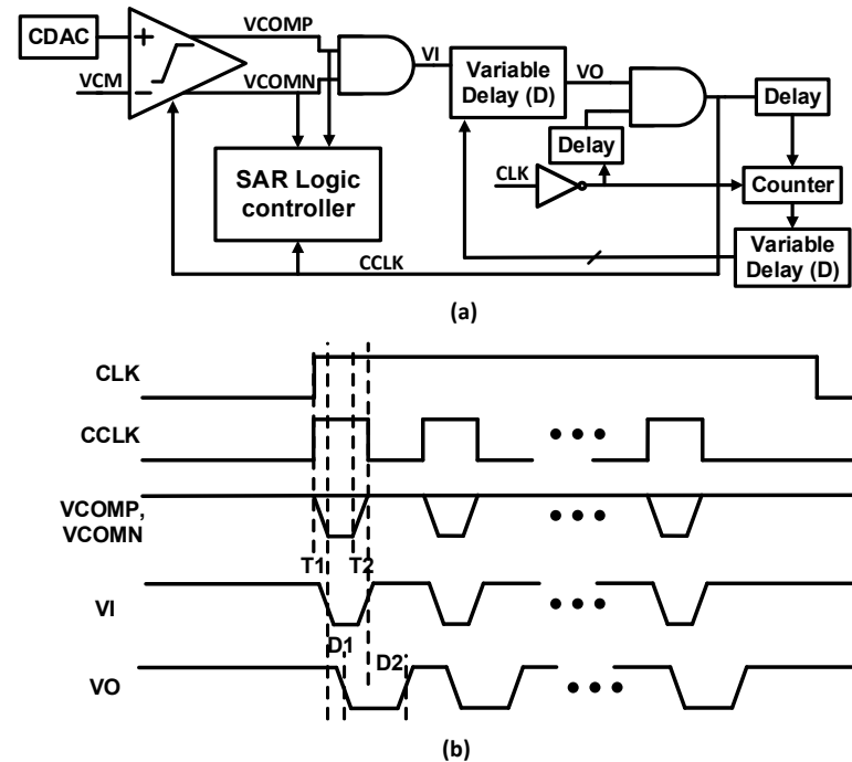
Figure 8. (a) Block diagram of the clock generator; (b) timing diagram of the clock generator.
