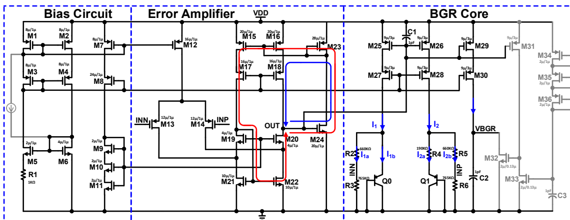
Figure 10. Schematic of BGR.
