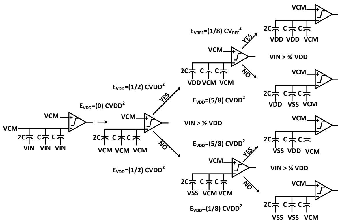
Figure 3. The proposed 3-bit switching method for single-input SAR ADC.
