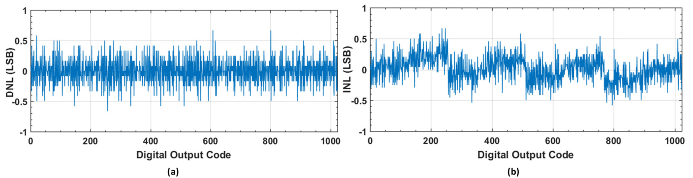
Figure 5. Static performance of the proposed switching with 1% unit capacitor mismatch. (a) DNL; (b) INL.
