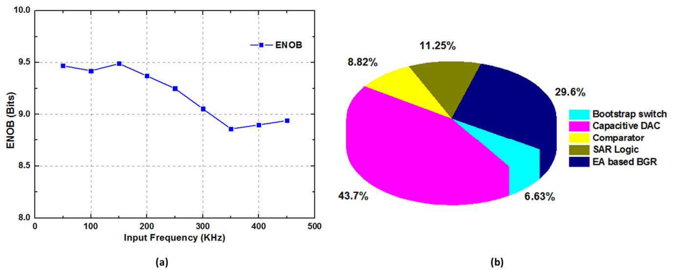
Figure 16. (a) Measured ENOB trend at different input frequencies with 1 MS/s sampling speed; (b) Power breakdown of proposed ADC.
