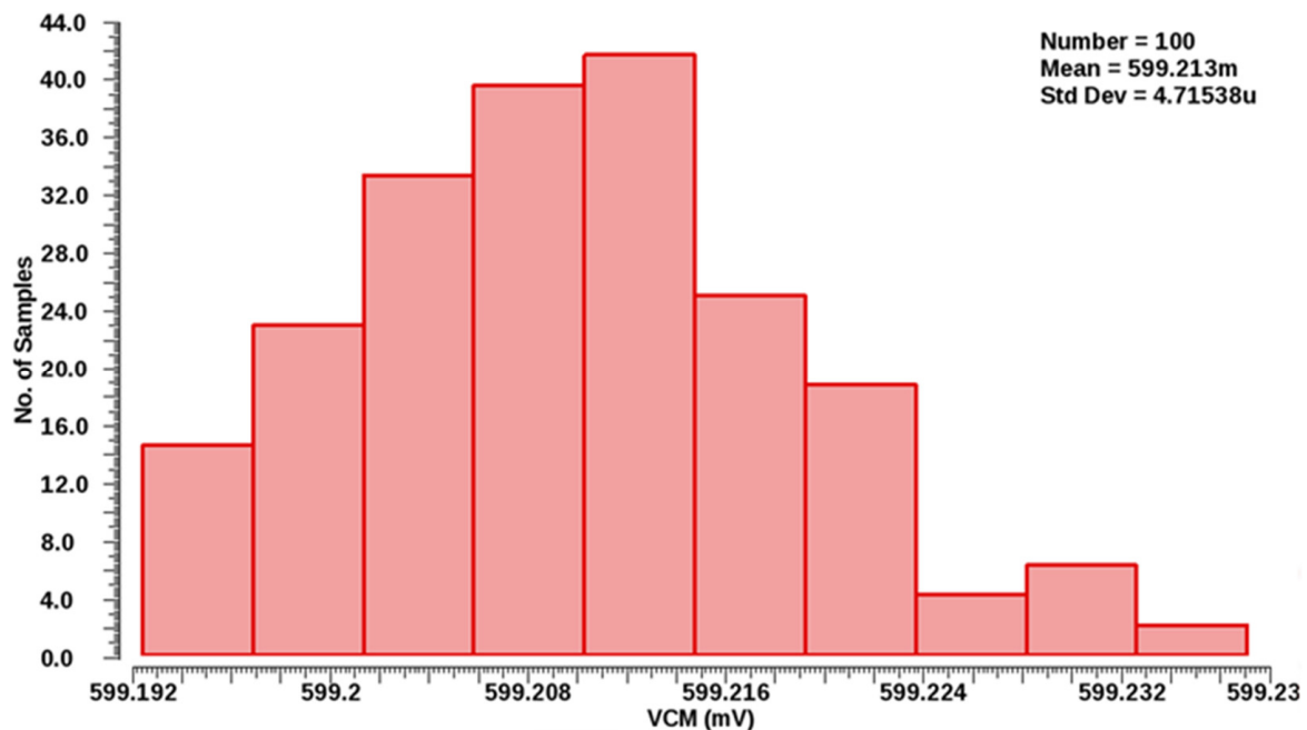
Figure 12. Monte Carlo simulation result of error amplifier-based bandgap reference voltage generator.
