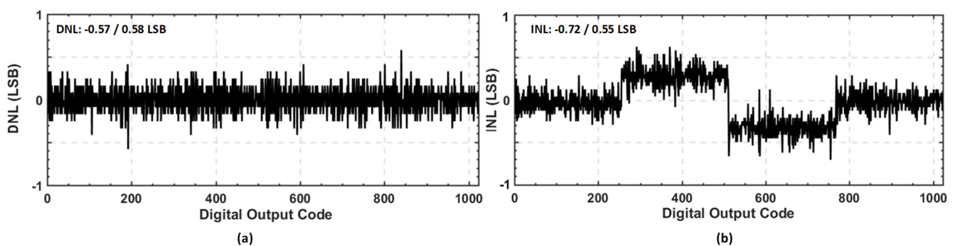
Figure 15. Measured static performance: (a) Differential non-linearity (DNL); (b) Integral non-linearity (INL).
