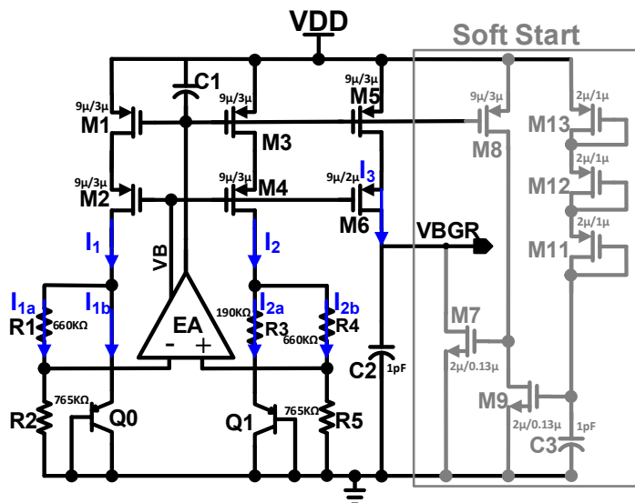
Figure 10. Schematic of BGR.
