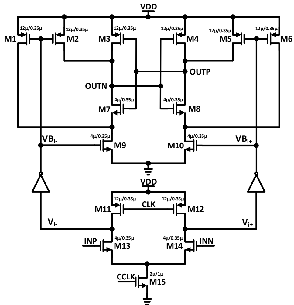
Figure 7. Transistor-level schematic of the dynamic comparator.
