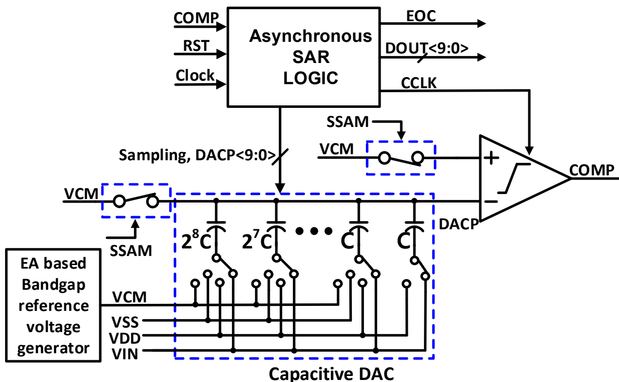
Figure 1. The proposed block diagram of the asynchronous SAR ADC with an EA-based bandgap reference voltage generator circuit.
