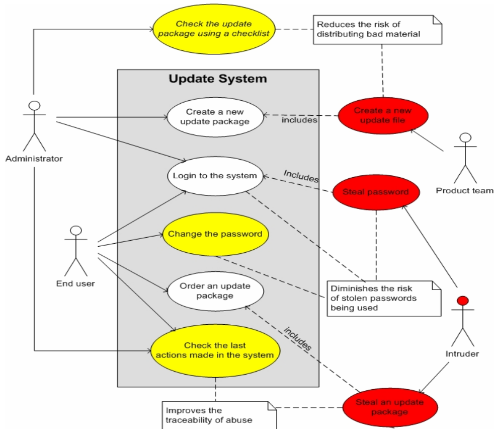
Figure 13. A use case diagram for the IS. The product team is an example of an insider threat and the intruder represents threat from outside. Four elements are red in color: “create a new update file,” “steal password,” “intruder,” and “Steal an update package.” Three elements are yellow in color: “Check the update package,” “Change the password,” and “Check the last actions.”
