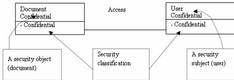
Figure 8. A Meta-notation enriched class diagram.
