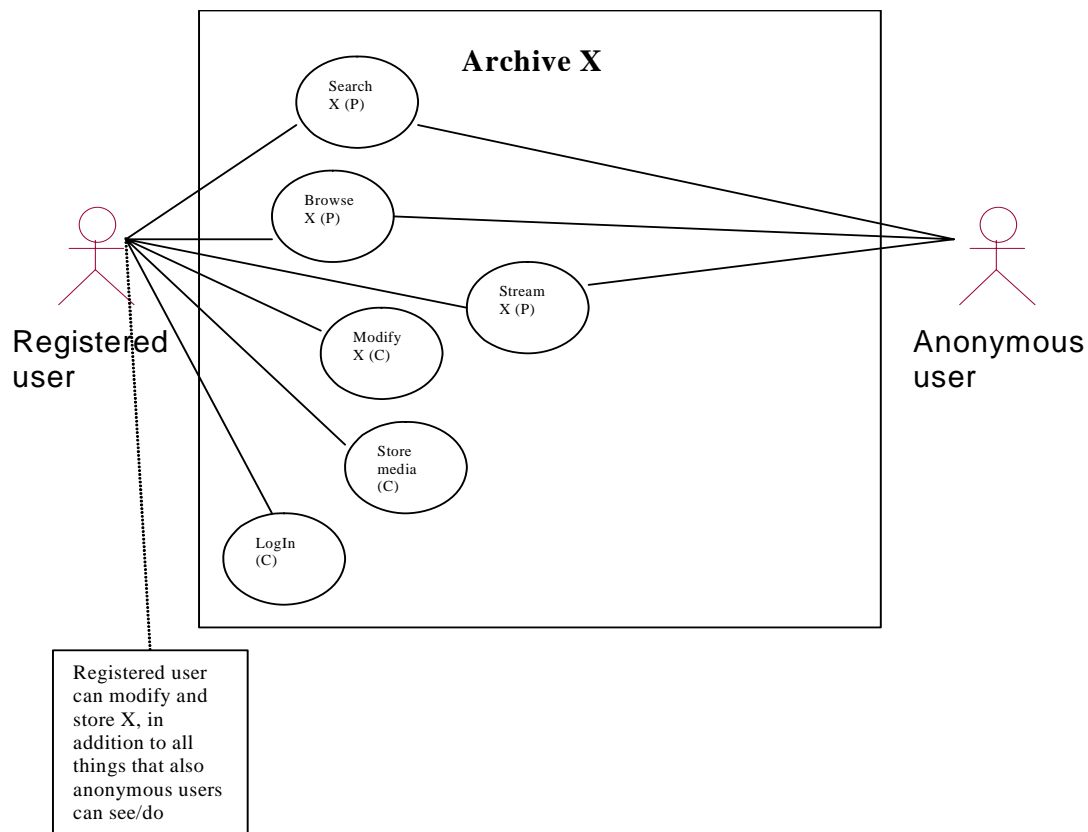
Figure 15. Modified example of “a second level use case” from the project.
