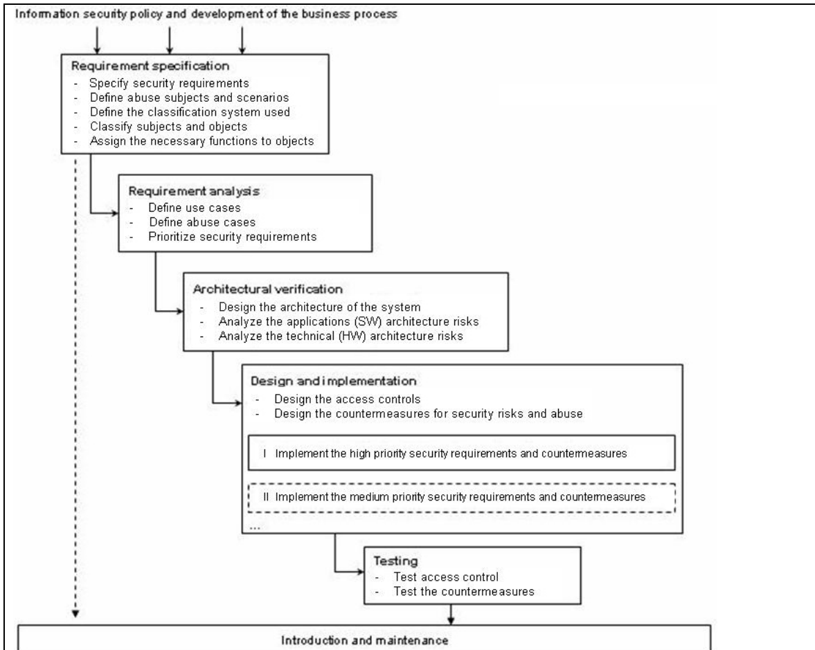
Figure 12. The Meta-notation enriched RAD process model after integration of the Meta-notation.
