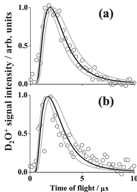
FIG. 5. (a) TOF spectrum of \text{D}_2\text{O}(v=0) formed by 157 nm photoirradiation of ASW( \text{D}_2\text{O} ) at 90 K, monitored by 2+1 REMPI via the line at 248.057 nm of the C-X 0_0^0 band. The solid curve is a fit to the data derived assuming T_{\text{trans}}=1800 K. (b) TOF spectrum of \text{D}_2\text{O}(v=0) formed by 193 nm photoirradiation of the \text{D}_2\text{O}:\text{H}_2\text{S} mixed ice sample at 90 K, monitored by (2+1) REMPI via the line at 247.865 nm, which is mainly the 1_{01}-2_{20} transition of the C-X 0_0^0 band. The solid curve is a fit to the data derived assuming T_{\text{trans}}=2250 K. The two gray curves show the range spanned by the error bars quoted in Table I.
