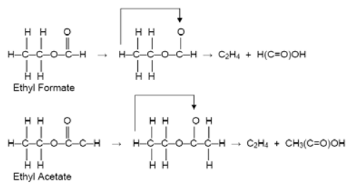
Figure 2 Schematic of molecular elimination reaction pathways for ethyl formate and ethyl acetate
